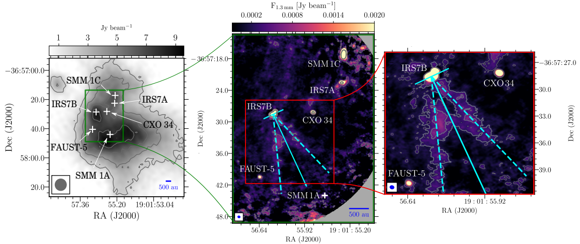
Fig. 1. Corona Australis cluster: left: SCUBA-2 map at 450 \mu\text{m} (JCMT archive). Contours are at [12, 18, 30]\sigma where 1\sigma = 0.3 \text{ mJy beam}^{-1} ; central: ALMA map of continuum emission at 1.3 mm. The first contour and steps are 6\sigma ( 0.48 \text{ mJy beam}^{-1} ) and 70\sigma , respectively. Right: Zoom onto IRS7B, where only the contours at [3, 6]\sigma are shown. The detected protostellar objects are labelled. SMM 1A is not detected at 1.3 mm. The cyan line shows the PA of the IRS7B system (i.e. 115^\circ ; see text), while the arrow indicates the perpendicular direction. Dashed lines follow the elongated structures detected at 3\sigma . The synthesised beam is shown in the bottom-left corner of each panel.
