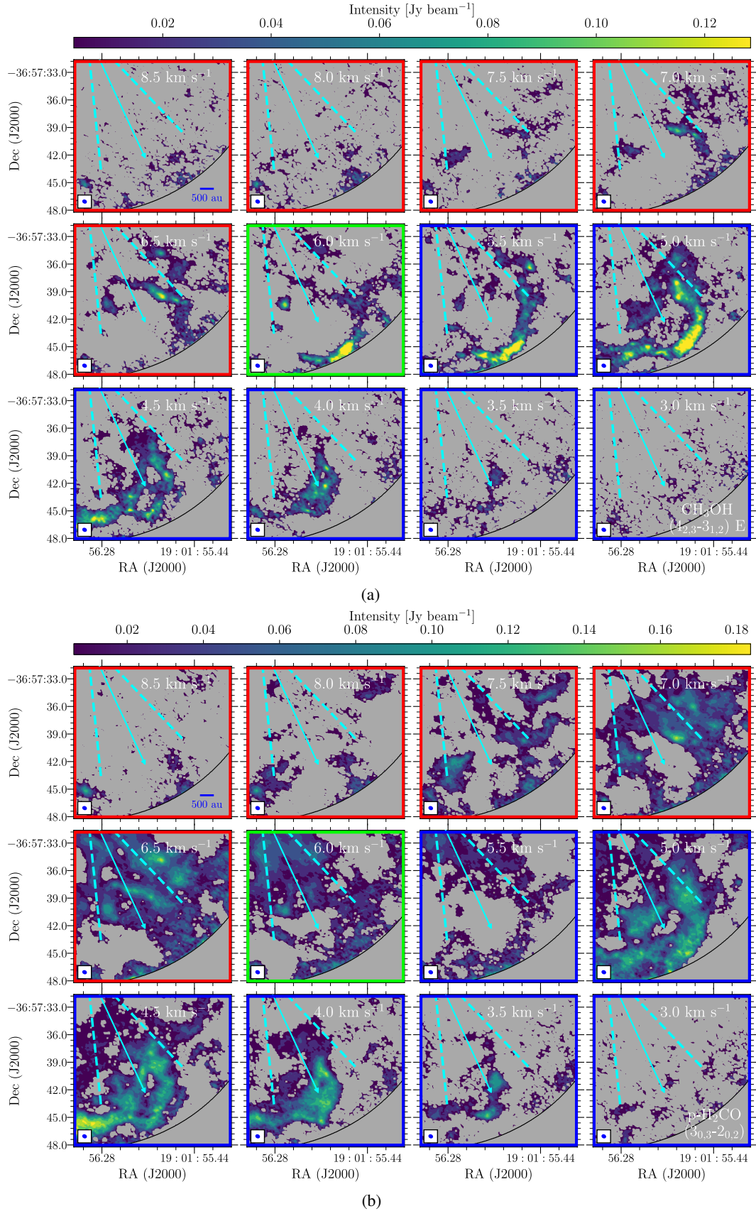
Fig. B.1. Velocity channel maps of (a) \text{CH}_3\text{OH} ( 4_{2,3}-3_{1,2} ) E and (b) p\text{-H}_2\text{CO} ( 3_{0,3}-2_{0,2} ). The green framed panel marks the systemic velocity of IRS7B, while the blue- and red- framed panels represent the blueshifted and redshifted components of the emission, respectively. The emission was masked at 3\sigma , and the colour bar peaks at 75\sigma , where the average 1\sigma noise in each channel is (a) 1.2 \text{ mJy beam}^{-1} and (b) 2 \text{ mJy beam}^{-1} . The black arc shows the ALMA Band 6 FoV. Each panel reports the corresponding velocity. (a) Channel map of \text{CH}_3\text{OH} ( 4_{2,3}-3_{1,2} ) E (b) Channel map of p\text{-H}_2\text{CO} ( 3_{0,3}-2_{0,2} )
