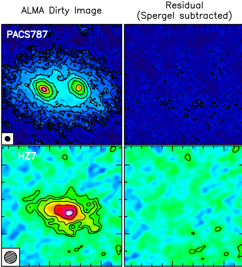
Fig. 15. Examples of ALMA images of CO(5–4) and [CII] emission from high- z star-forming galaxies PACS-787 (top) and HZ7 (bottom). Left: ALMA dirty image. Right: residual map with the primary disk component modeled by a single Spergel profile subtracted. The image size is 3.5'' \times 3.5'' . The synthesized beam ( 0.15'' \times 0.14'' and 0.36'' \times 0.35'' for PACS-787 and HZ7, respectively) is presented in the bottom left of the left panels. Contours start from \pm 2\sigma and increase by a factor of 1.5.
