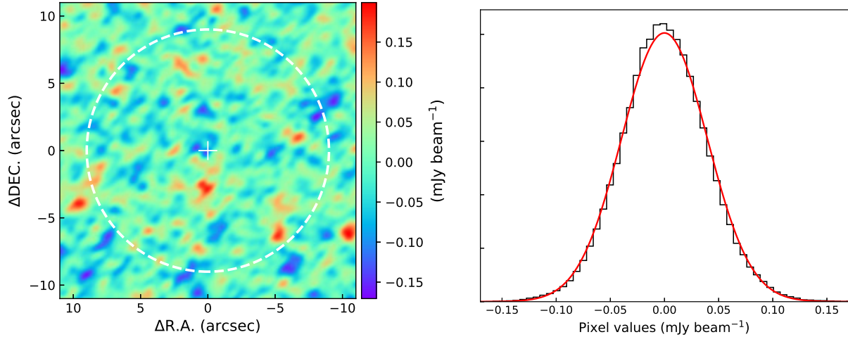
Fig. 4. Example of an empty dataset used for our simulations. Left: noise map. The source emission (which was close to the phase center) was subtracted from the visibility data. The dashed white circle represents the primary beam (i.e., the FOV) of the dataset. Right: histogram of pixel values within the primary beam. The red line represents the best-fitting Gaussian model. The fit suggests that the noise data is at least approximately Gaussian.
