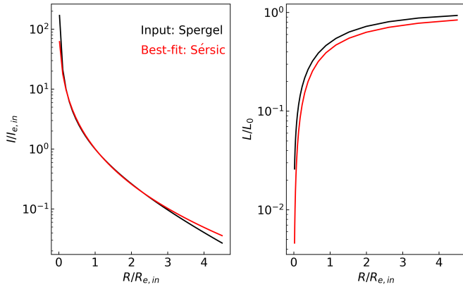
Fig. A.1. Comparison of the Sérsic profile with the Spergel profile using mathematical simulations. Left: Surface density profiles for Spergel function (black) compared to the best fit with a Sérsic function (red) through mathematical simulations. Right: Comparison of the integrated surface density profiles for the Sérsic and Spergel functions shown in the left panel. The values of R_{e,in} and I_{e,in} are held fixed and represent the input parameters in the Spergel profile.
