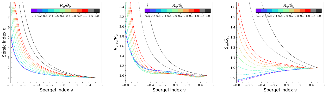
Fig. A.2. Comparison between Spergel index \nu and Sérsic index n (left), the ratio of R_e (middle) and total flux (right) obtained from the profile fitting using a Sérsic function to the input value in the Spergel model as a function of Spergel index \nu .
