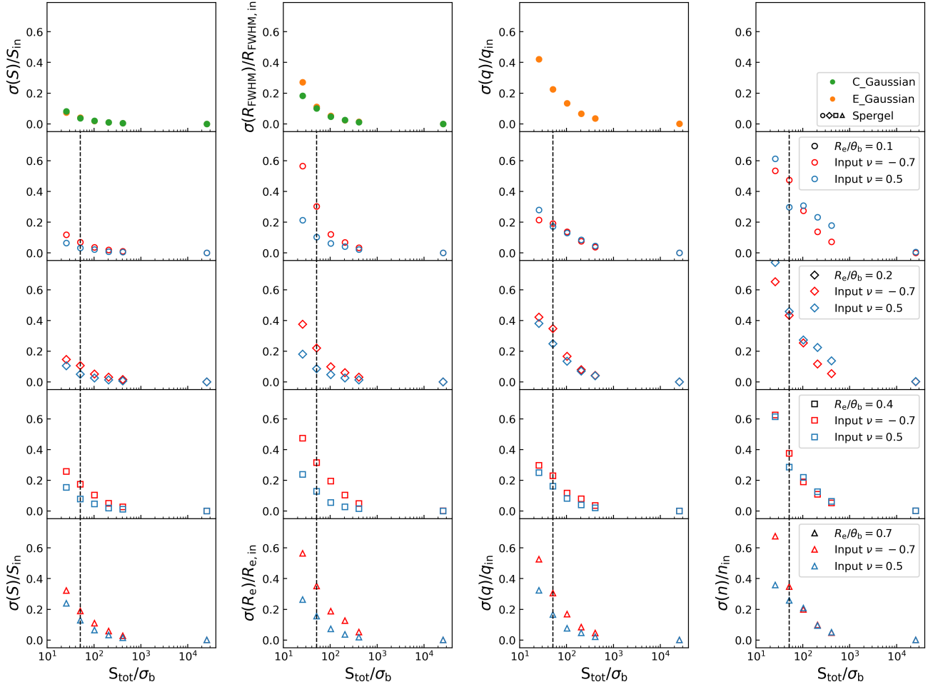
Fig. 9. Relative accuracy of the uv -based parameter estimates, flux density, effective radius, axis ratio, and Sérsic index (from left to right) given by \sigma(\text{para})/\text{para} . Here, \sigma(\text{para}) is the uncertainties of the parameter estimates distribution and is calculated as 1.48 \times \text{MAD} , as a function of the S/N of flux density. The top panels show the results derived from fits with an elliptical Gaussian (orange) and circular Gaussian (green) model, while the results from a Spergel model uv fit with input R_e/\theta_b of 0.1, 0.2, 0.4, and 0.7 are shown in panels from the second to fifth rows, respectively. We only display results for the cases with a Spergel index of 0.5 and -0.7 from our simulation. For other cases with a Spergel index between \nu = 0.5 and -0.7 , the results were found to be within or close to those shown in the panels between the second and fifth rows. The dashed vertical lines represent the threshold of S_{\text{tot}}/\sigma_b of 50.
