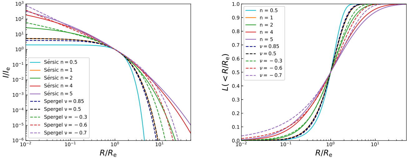
Fig. 1. Comparison of surface density profiles (left) and the cumulative distributions (right) for Sérsic (solid lines) and Spergel (dashed lines) functions. The light profile with a Sérsic index of 0.5, 1, 2, 4, and 5 and a Spergel index of 0.85, 0.5, -0.3 , -0.6 , and -0.7 is shown in different colors. By definition, R_e contains half of the integrated galaxy light.
