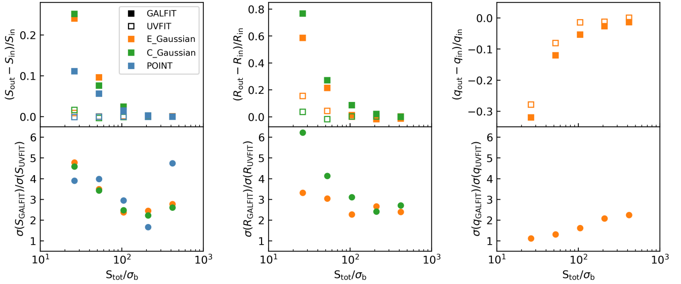
Fig. 12. Comparison of profile fitting of Gaussian and PSF models in the uv -plane and the image plane. Top: relative difference between recovered and input parameters of flux density (left), size (middle), and axis ratio (right). The recovered parameters were obtained from fitting with an elliptical Gaussian (orange), a circular Gaussian (green), and a point (blue) source model using uv_fit (open symbols) and galfit (solid symbols). Bottom: similar to the top panels, but we plot the ratio of measurement uncertainty derived from galfit in the image plane to that obtained from uv_fit in the uv -plane. The measurement uncertainties are estimated as \sigma = 1.48 \times \text{MAD} .
