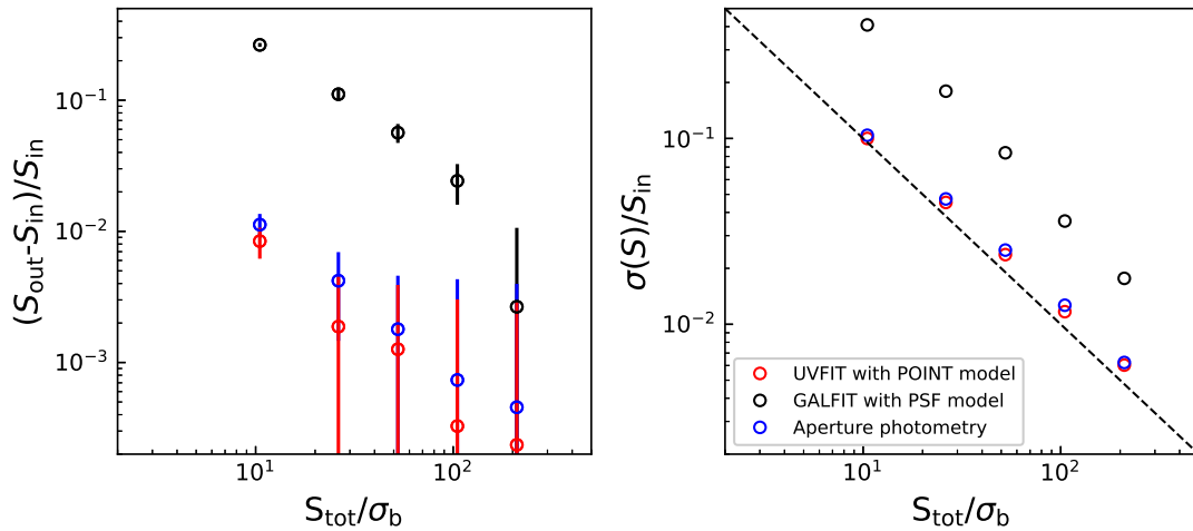
Fig. 13. Simulation results of the flux density bias (left) and relative uncertainty of measurement on the recovery of flux density (right) for point sources using uv_fit (red), galfit (black), and aperture photometry (blue) in the image-plane fitting, as a function of the flux S/N . The error bars in the left panel represent the standard error on the mean. The dashed line in the right panel is a 1:-1 line.
