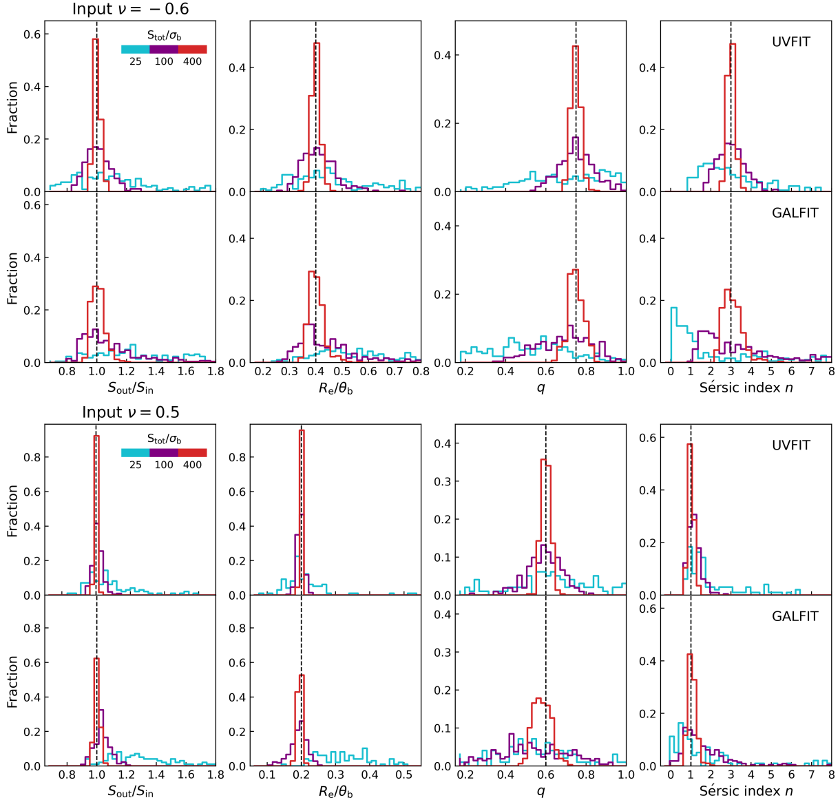
Fig. 6. Results from simulations of a single model source. The distribution of recovered parameters from uv_fit to the visibilities (panels labelled with UVFIT) and galfit in the image plane (panels labelled with GALFIT) allowed us to measure their respective accuracy in recovering the known intrinsic parameters (dashed vertical lines), including the flux density and structural parameters ( R_e , q , and n ). We present two examples using a Spergel profile as the input source: R_e/\theta_b = 0.4 , q = 0.75 , PA = 30^\circ , \nu = -0.6 (two top panels), and R_e/\theta_b = 0.2 , q = 0.6 , PA = 30^\circ , \nu = 0.5 (two bottom panels). The distribution of the recovered parameters is color coded by flux density ( S_{\text{tot}}/\sigma_b = 25, 100, \text{ and } 400 , indicated by different colors in the inset panel). The Sérsic indices shown in the UVFIT panels were obtained by converting the best-fit Spergel indices based on Eq. (3). For all parameters, we took into account the conversion from Spergel-based fits to Sérsic-based fits, discussed in Sect. 2 (see Eqs. (3) and (4)), to remove any underlying systematics coming from the difference in the profiles.
