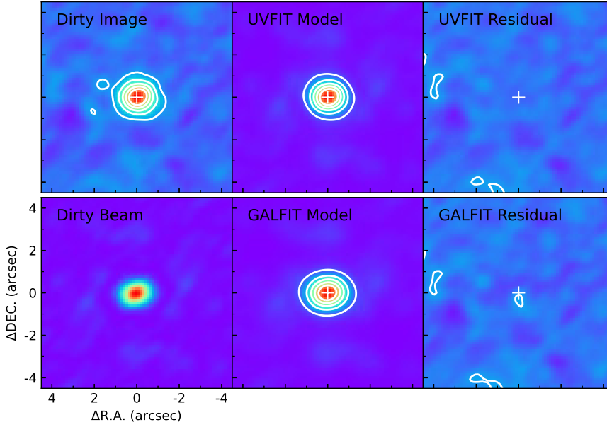
Fig. 5. Example of a simulated source generated with a Spergel profile of S_{\text{tot}}/\sigma_b = 50 , R_c/\theta_b = 0.4 , axis ratio of q = 0.75 , \text{PA} = 30^\circ , and Spergel index of \nu = -0.6 . From left to right: the dirty image (top-left), dirty beam (PSF used for convolution in galfit; bottom-left), best-fit source models convolved with the dirty beam (middle), and residuals after subtracting the model source (right). The model source and the model-subtracted residual shown in the top and bottom rows were derived from the uv_fit and galfit fits, respectively. Each image cutout is 9'' \times 9'' . The contours start from 2\sigma and increase in steps of 4\sigma . White crosses mark the best-fit source position obtained from uv_fit .
