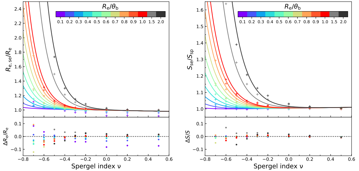
Fig. 3. Similar to Fig. 2 but showing the ratio of effective radii (left) and total fluxes (right) obtained from fitting Sérsic models to simulated galaxies created using Spergel profiles (crosses). The data are plotted as a function of their Spergel index. The solid curves denote the best-fit empirical relations as expressed by Eq. (4). The bottom panels show the normalized residuals to the best fit, which are largely within 10%.
