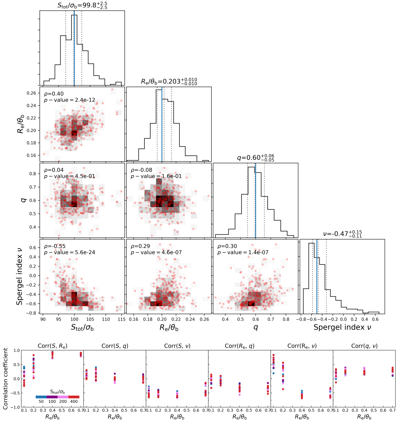
Fig. 11. Correlations between the fitted parameters obtained from Spergel profile fitting in the uv -plane. Top: corner plots showing the covariances between the free parameters modeled in the Spergel profile fitting. The example model source has a flux density of S_{\text{tot}}/\sigma_b = 100 , a size of R_e/\theta_b = 0.2 , an axis ratio of q=0.6 , and a Spergel index of \nu = -0.5 . The shaded density histograms show the two-parameter distributions with the Spearman rank correlation coefficient and p -value marked in each panel. The one-dimensional histograms at the top of each column represent the individual parameter distributions, annotated with the median values. The boundaries of the 25th and 75th percentiles of the distribution are plotted as dashed lines, while the blue vertical lines show the true values. Bottom: Spearman's rank correlation coefficients of the two-parameter pairs as a function of source size. The points are color coded by the input flux density.
