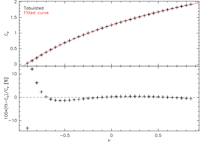
Fig. C.1. Comparison between tabulated values of the c_\nu function with an analytical approximation.
