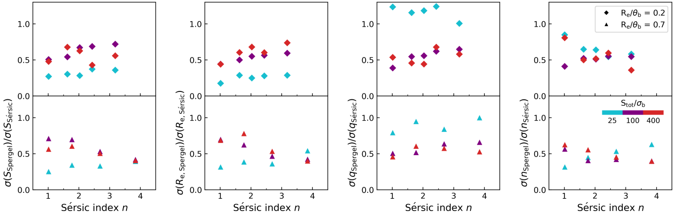
Fig. 8. Similar to Fig. 7, but we plot the ratio of the scatter of the measurements derived from Spergel fits in the uv -plane to that derived from Sérsic fits in the image plane for fitted parameters. From left to right, we show the flux density, effective radius, axis ratio, and Sérsic index as a function of light concentration (i.e., Sérsic index).
