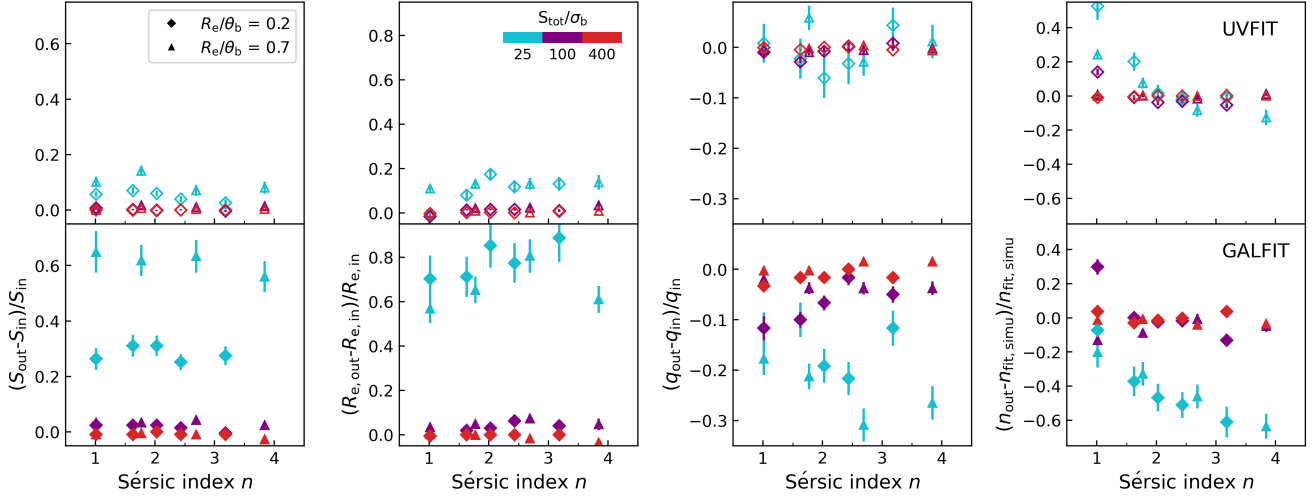
Fig. 7. Relative difference between the input and measured parameters, flux density, effective radius, axis ratio, and Sérsic index (from left to right) obtained from Spergel fits to the uv -plane (top panels) and Sérsic fits in the image plane using galfit (bottom panels) in our simulations plotted as a function of light concentration (i.e., Sérsic index) for various S_{\text{tot}}/\sigma_b and source sizes. Sources with a size of R_e/\theta_b = 0.2 and 0.7 are marked by a diamond and a triangle, respectively, while the inset panel's color bar shows the different input flux densities. The error bars denote the interquartile range of the distribution divided by the square root of the number of simulations.
