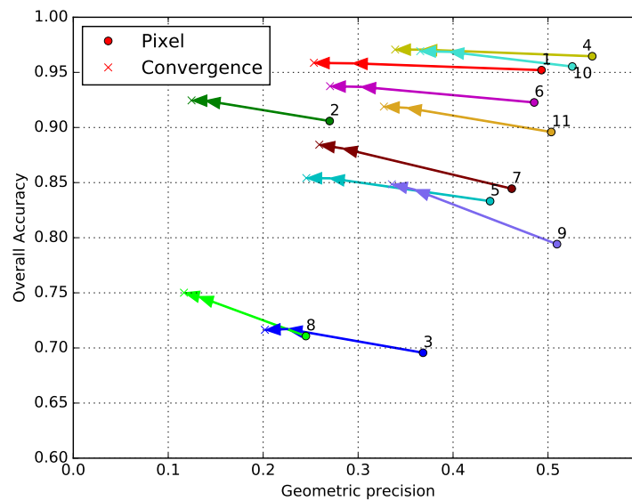
Figure 10. Iterations of the HACCS process. The arrows represent successive iterations, which start from the pixel-based classification, and reach the convergence point once no significant change is detected. The numbers and colors represent the different tiles, once again following the definitions from Table 2.
