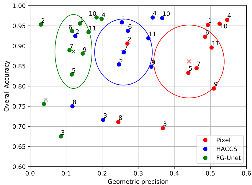
Figure 12. Statistic accuracy and geometric accuracy of the pixel based classification, of HACCS, and of the FG-Net (CNN) on eleven tiles of the Sentinel-2 data set. The number labels designate the tile that was used for training and testing, the correspondence is given in Table 2.
