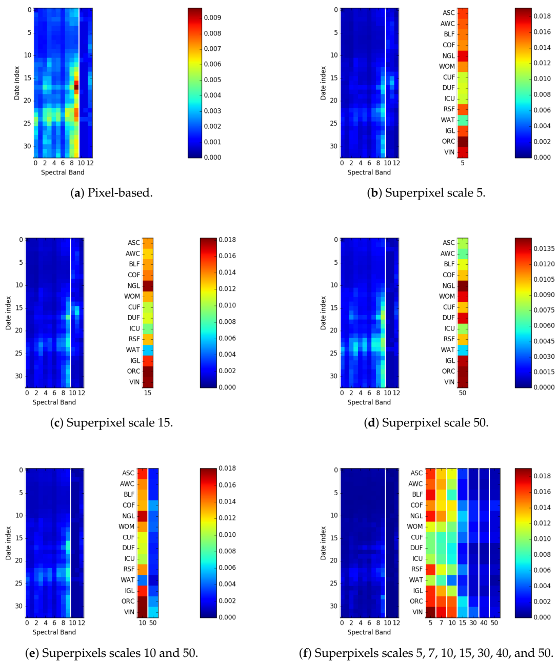
Figure 13. Evolution of the RF variable importance for different superpixel scales and combination of scales, after 3 iterations of HACCS. In each figure, the importance of the pixel features is shown on the left side, organized by date index and spectral band. A red color indicates a feature with a high importance. The dates cover a period of the year 2016, starting in January. The importance of the histogram of the local classes features in superpixels are shown on the right side of each feature, and are organized according to the scale of feature and the associated class. It appears that the semantic contextual features were indeed considered important by the RF, and that when more than one scale was provided, the local scales provided more important contextual information.
