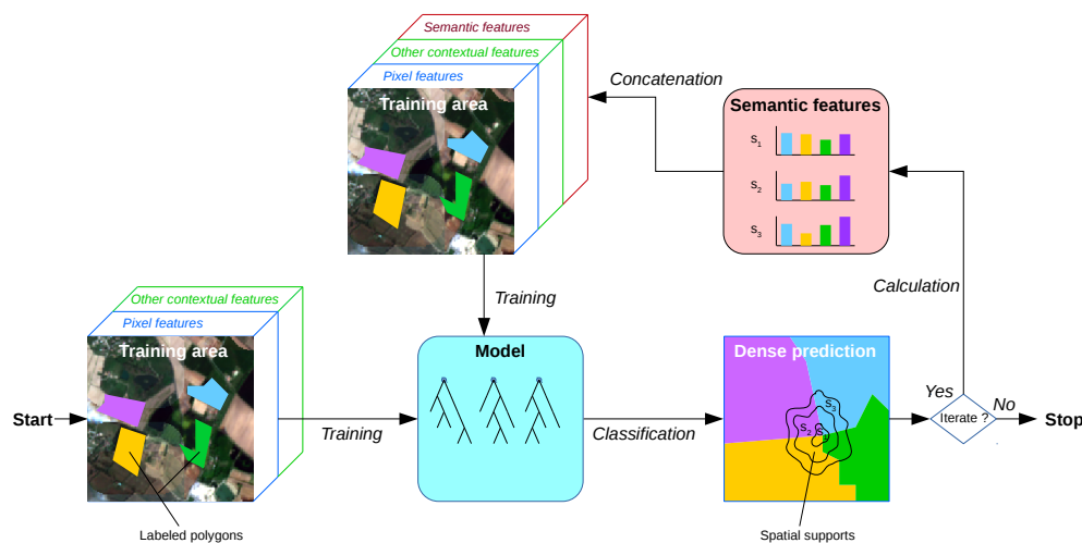
Figure 1. The Histogram of Auto-Context Classes in Superpixels process. A dense labeling of all the pixels is used to compute the histogram of the different classes. This histogram provides a contextual characterization, which serves as a supplementary feature for the next classification step, to refine the decision based on nearby contextual cues. The initial dense prediction can also originate from a different classification system, such as a Convolutional Neural Network (CNN).
