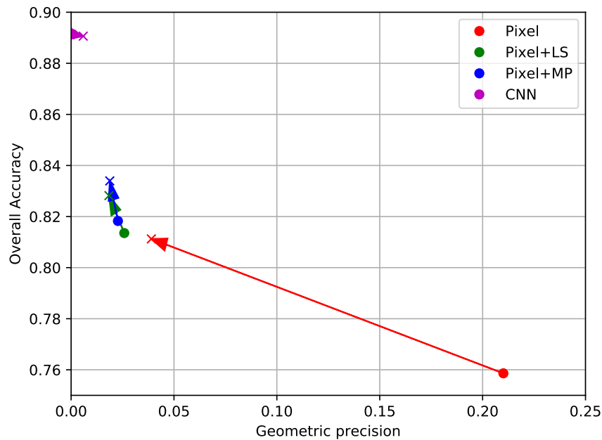
Figure 17. OA and PBCM of the different methods compared in Table 6. The solid points show the iteration 0, in other words, the scores of the method used to generate the classification map for the first class histograms. The arrows show the evolution after four iterations of HACCS, with a cross indicating the convergence point.
