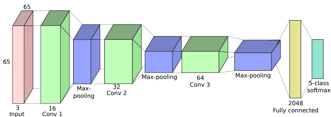
Figure 3. Architecture of the patch-based network that is used for comparison with the Histogram of Auto Context Classes in Superpixels (HACCS), identical to the work in [50]. The first layer intakes a neighborhood of 65 \times 65 pixels around the central pixel. Then, this relatively shallow network contains three stages of convolution and max-pooling, followed by a fully connected layer.
