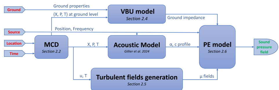
Figure 2. Architecture of the model used in this study. It shows how to use the MCD (Martian Climate Database) to retrieve the atmosphere chemical composition X , wind speed u , pressure P and temperature T and feed them into the model presented in Gillier et al. (2024) to compute sound speed c and attenuation \alpha in the atmosphere. The VBU (Venegas-Boutin-Umnova) model is used to predict porous regolith effects on acoustic waves, and the PE (Parabolic Equation) to obtain the overall sound field. The process of generating turbulent field of the refractive index \mu is described in Section 2.5.
