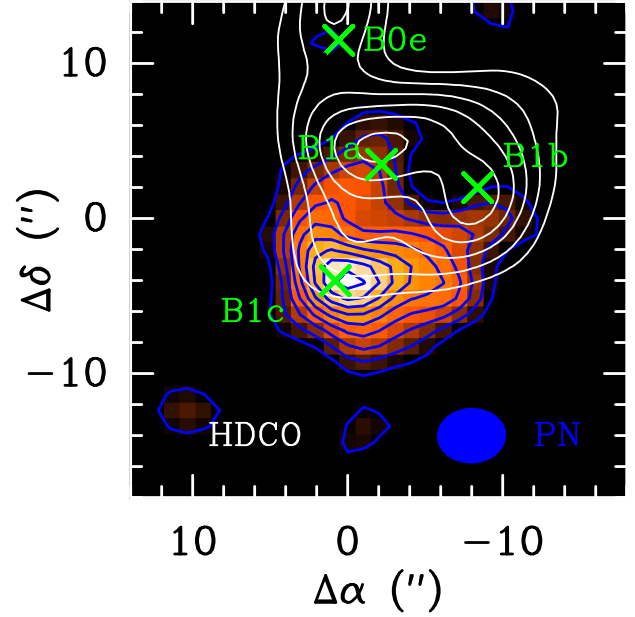
Fig. 7. Comparison of the PN N = 2-1 and HDCO J = 2-1 flux distributions. The PN N = 2-1 line flux (colourscale and blue contours) is integrated in the velocity interval [-11; +4.6] \text{ km s}^{-1} ; the first contour and contour interval are 3\sigma ( 2.8 \times 10^{-2} \text{ Jy beam}^{-1} \text{ km s}^{-1} ) and 2\sigma ( 1.8 \times 10^{-2} \text{ Jy beam}^{-1} \text{ km s}^{-1} ), respectively. The synthesized beam of the PN N = 2-1 is depicted by a blue ellipse in the bottom right corner. The HDCO J = 4_{1,4}-3_{1,3} emission (white contours) is integrated in the velocity interval [-0.7; +3.4] \text{ km s}^{-1} ; the first contour and contour interval are 20% and 15% of the peak intensity, respectively. The map was smoothed down to the angular resolution of the PN N = 2-1 line. The HDCO J = 2-1 data are from Fontani et al. (2014). Coordinates are in arcsecond offsets with respect to the nominal position of L1157-B1.
