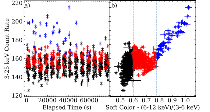
Figure 9. (a) 3–25 keV NuSTAR light curve (combined FPMA and FPMB); (b) 3–25 keV count rate vs. soft color, defined as the ratio of counts in the 6–12 keV and 3–6 keV bands. All data points are constructed from 64 s bins. The black, red, and blue data points corresponding to different spectral branches for which we investigated the cospectral properties—see Table 3 for the best-fit parameters to the (temporal) cospectra.
