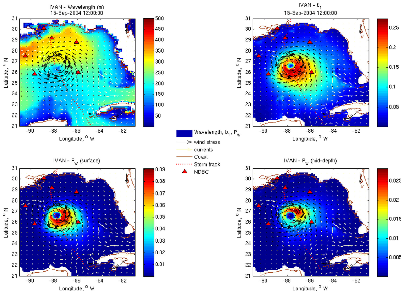
Figure 7. (top left) Wavelength; (top right) variability of b_1 = 5 \left(\frac{H}{L}\right)^2 in Exp. M7; (bottom left) turbulence production due to nonbreaking waves ( P_w ) at the surface; and (bottom right) P_w at middepth on 15 September 2004 1200 during Hurricane Ivan.
