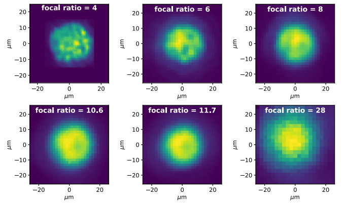
Fig. 8. Coupling maps acquired for various focal ratios at a fixed wavelength of 765.5 nm.
