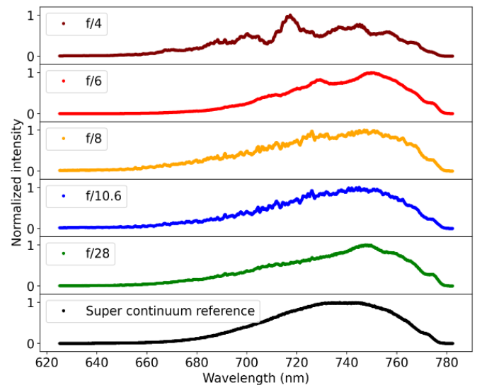
Fig. 12. Supercontinuum spectrum reconstructions from PL data at various focal ratios. Each spectrum is normalized by its maximal value. The spectra can be compared to the reference on the bottom plot, obtained with an SMF.
