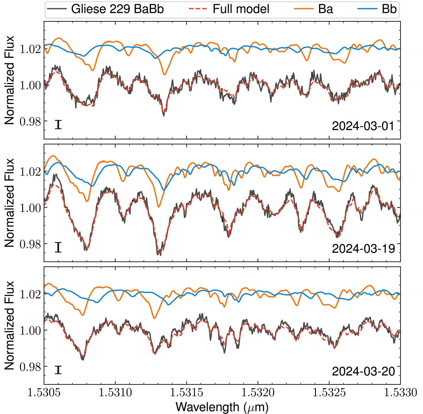
Extended Data Fig. 4 | Zoom-in of the CRILES+ spectra of Gliese 229 B on three different nights. A small portion of the CRILES+ spectra on three different nights on which we achieve the highest S/N (black). The Ba and Bb models are shown in orange and blue, respectively, and the full model is in red. The median uncertainties for the spectra are denoted as error bars at the lower
