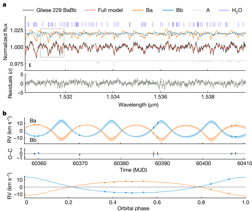
Fig. 2 | CRIRES+ spectrum and spectroscopic orbit of Gliese 229 Ba and Bb. a , A segment of the CRIRES+ spectrum from 20 March 2024 (black) used to compute RVs of Gliese 229 Ba and Bb. The region is dominated by water-absorption lines from the brown dwarfs, whose positions are marked in purple. The orange and blue curves are spectral models for Ba and Bb, respectively, and the dashed grey curve is the CRIRES+ spectra of Gliese 229 A used to model stellar contamination. The three model components have been offset for clarity. The full model is shown in red. The median uncertainty of the spectrum is
