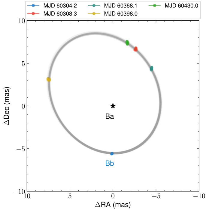
Extended Data Fig. 6 | Relative orbit of Gliese 229 Bb with respect to Gliese 229 Ba from GRAVITY and CRILES+. Random draws of the relative astrometric orbit of Gliese 229 Ba-Bb from the PMOIRE fit are shown as grey curves. The position of the primary brown dwarf Gliese 229 Ba is marked with a star at the origin. The coloured points show random draws of the predicted astrometric positions of Bb with respect to Ba from the joint GRAVITY and CRILES+ orbit fit over the five observing epochs.
