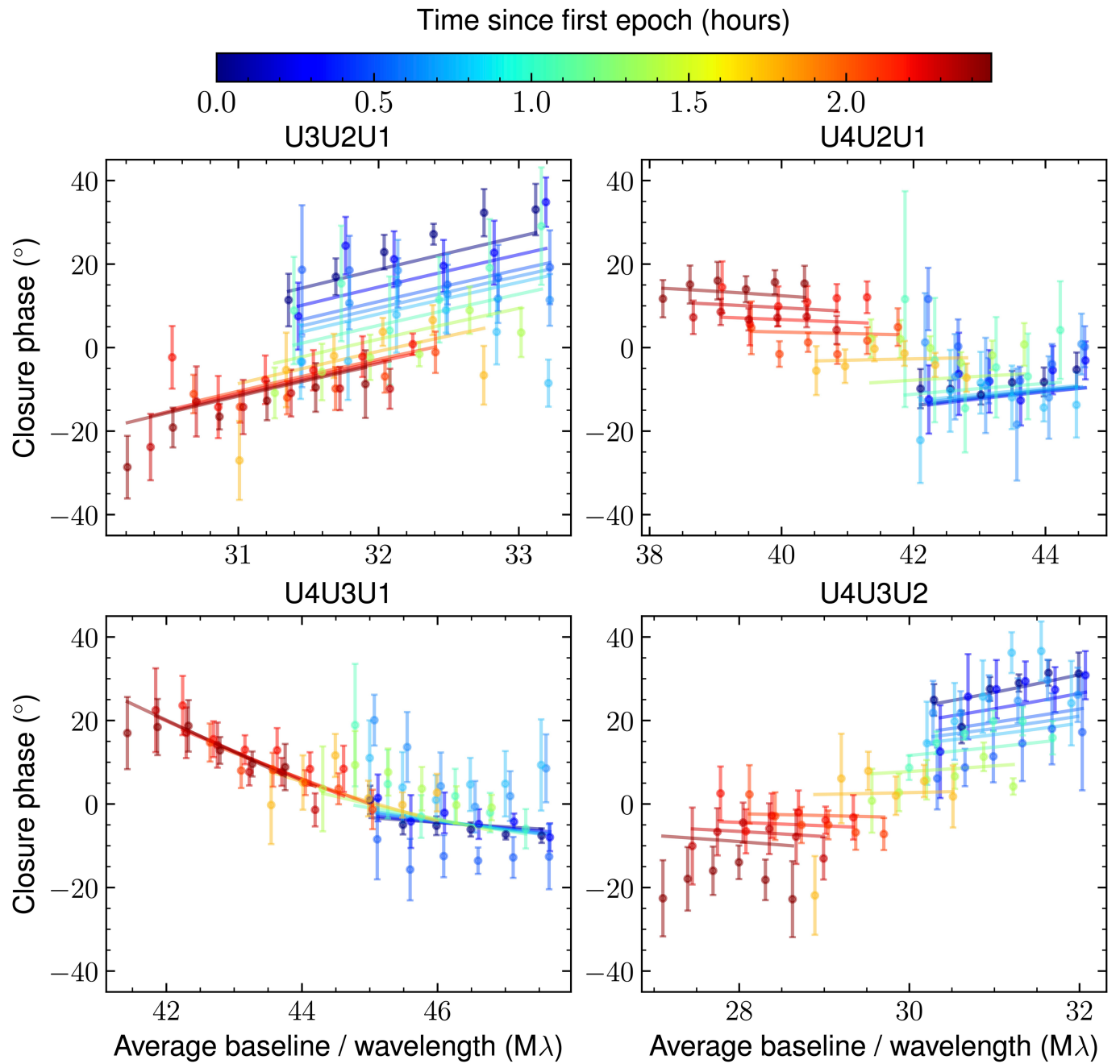
Extended Data Fig. 2 | GRAVITY closure phase measurements of Gliese 229 BaB on 26 December 2023. The GRAVITY closure phase measurements in the first epoch (26 December 2023). The data are in points and the models are shown as lines. Each panel is for a different baseline triangle between the four
