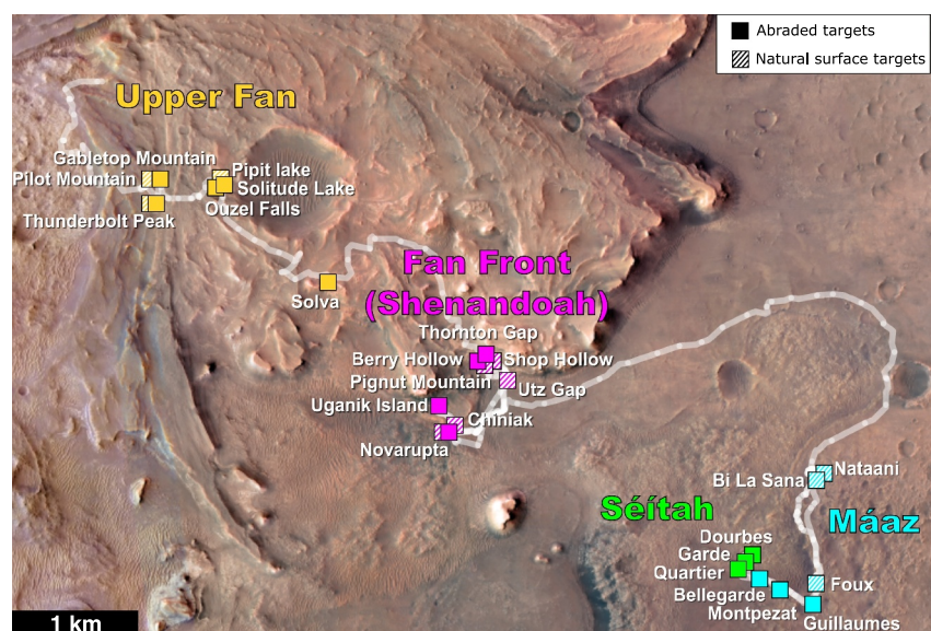
Figure 1. Locations of all SHERLOC bedrock targets analyzed in this work from the four regions: the Séítah formation, the Mááz formation, the sedimentary western fan front (Shenandoah formation), and the upper fan.
