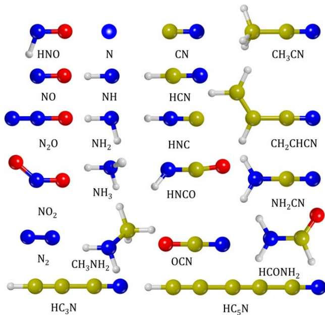
Figure 1. Set of N-bearing species considered in this work. Green represents carbon atoms, blue nitrogen, red oxygen, and gray hydrogen.
