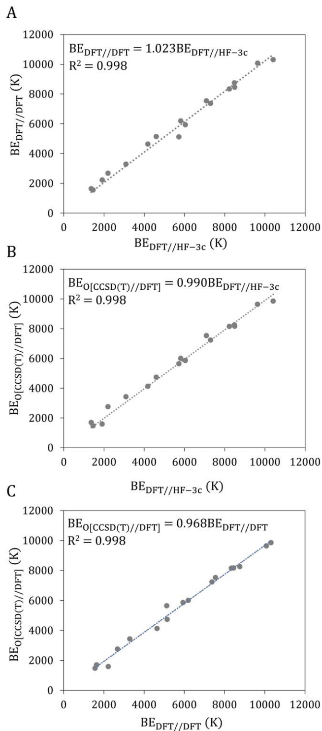
Figure 4. Linear fits between (A) the BE values computed at DFT//DFT vs. those at DFT//HF-3c level, (B) the BE values computed at O[CCSD(T)//DFT] level vs. those at DFT//HF-3c level, and (C) the BE values computed at O[CCSD(T)//DFT] level vs. those at DFT//DFT level. The linear fit equations are shown in the graphs.
