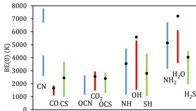
Figure 8. Comparison of BE(0)s for selected di-atomic and tri-atomic N-bearing species and their oxygen and sulfur analogs (Ferrero et al. 2020; Perrero et al. 2022; see text). Solid lines cover the ranges between the minimum and maximum BE(0)s computed on the ASW at DFT//HF-3c for N- (blue), O- (red), and for S- (green) bearing species. The range of BE(0)s for the CN species is divided between cases in which a hemibond is formed (top range) and those in which a hemibond is not formed (bottom range). For reference, also the BE(0)s on the CWS computed at DFT//HF-3c level are reported (filled black circles).
