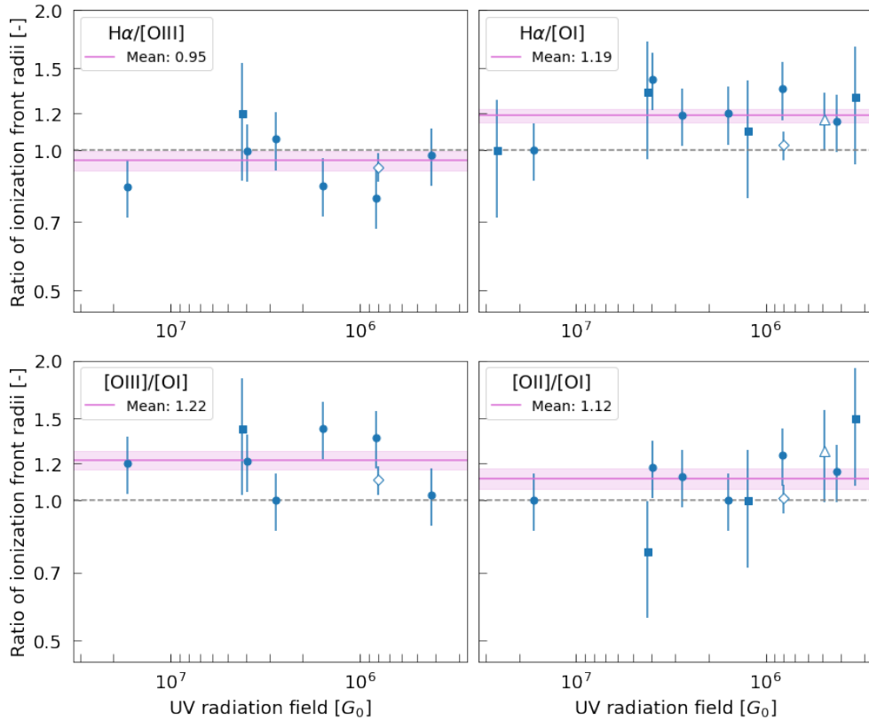
Fig. 7. Ratios of ionization front sizes of H \alpha , [O III], [O II], and [O I] as a function of the incident UV field. The empty diamond marks 244–440, and the empty triangle marks 203–504. The mean and SEM are marked in violet.
