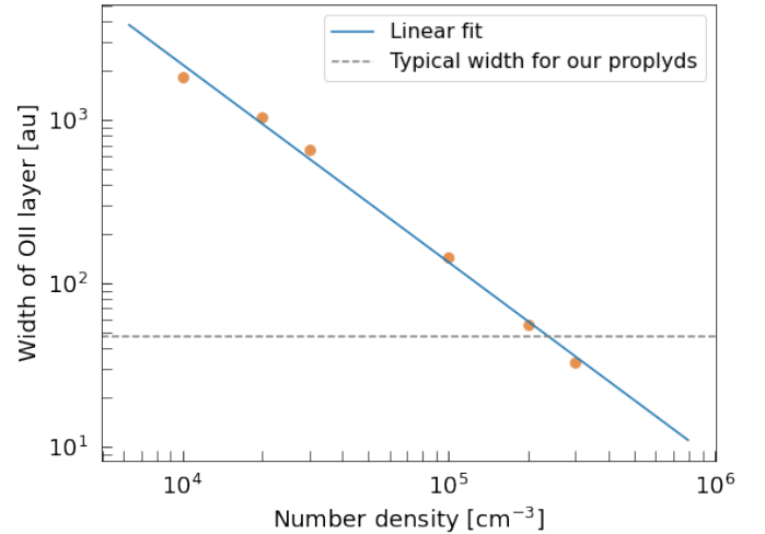
Fig. 11. Distance between the O III-O II transition and the O II-O I transition for a proplyd at a distance of 0.1 pc from a \theta^1 Ori C like star, as a function of the density in the cometary cusp of the proplyd. For densities \sim 2\text{--}3 \times 10^5 \text{ cm}^{-3} the thickness of the O II layer is consistent with our observations of ONC proplyds.
