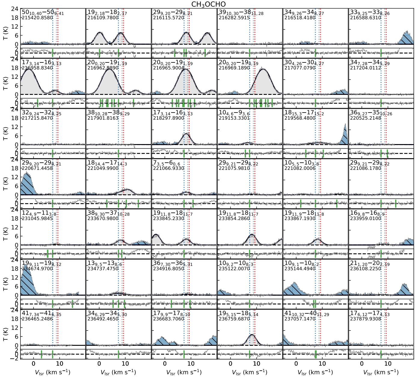
Fig. B.6. Same as Fig. B.2 but for CH 3 OCHO.
