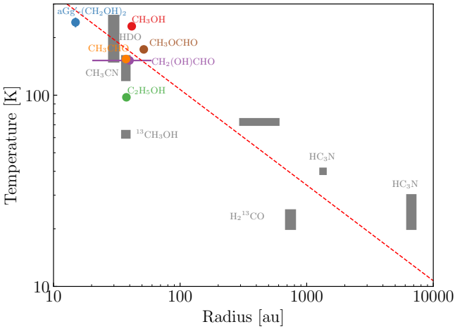
Fig. 8. Figure 9 from Bianchi et al. (2022a) with data points of COMs from this work.
