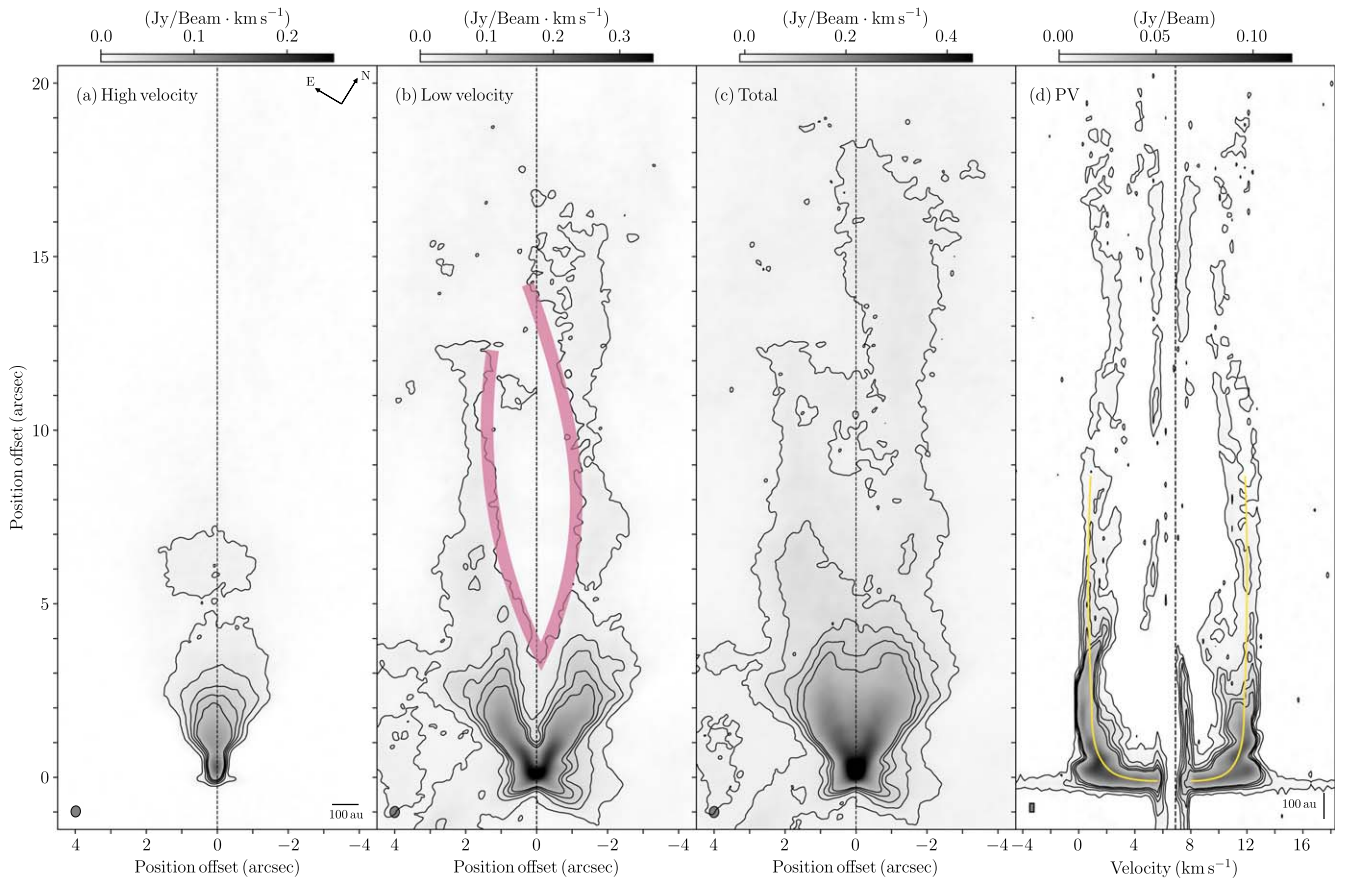
Figure 3. ALMA moment zero of the molecular outflow associated with HH 30 integrated over different ranges of the line-of-sight velocity. (a) High velocities, from -0.1 to 2.3 \text{ km s}^{-1} and from 11.3 to 14 \text{ km s}^{-1} . (b) Low velocities, from 2.6 to 11 \text{ km s}^{-1} . (c) Full range of the emission, from -0.1 \text{ km s}^{-1} to 14 \text{ km s}^{-1} . (d) Position–velocity diagram along the jet axis. The synthesized beam of panels (a), (b), and (c) is shown in the lower left corner. The magenta line in panel (b) traces an internal cavity of the molecular outflow. The yellow lines in panel (d) indicate the convex spur structure, and the gray bar represents the angular resolution ( 0''.3 or 42 \text{ au} ) and the channel width ( 0.3 \text{ km s}^{-1} ) used for the position–velocity cut. The contour levels in panels (a)–(c) start from 3\sigma with steps of 3\sigma , 6\sigma , 9\sigma , and 12\sigma , where (a) \sigma = 3.69 \times 10^{-3} \text{ Jy beam}^{-1} \text{ km s}^{-1} , (b) \sigma = 3.93 \times 10^{-3} \text{ Jy beam}^{-1} \text{ km s}^{-1} , and (c) \sigma = 5.87 \times 10^{-3} \text{ Jy beam}^{-1} \text{ km s}^{-1} . The contour levels in panel (d) start from 3\sigma with steps of 6\sigma , 12\sigma , 18\sigma , and 24\sigma , where \sigma = 9.62 \times 10^{-4} \text{ Jy beam}^{-1} .
