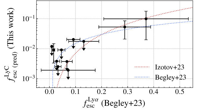
Figure 8. The comparison of the f_{\text{esc}}^{\text{LyC}} derived using the simulation and the Ly \alpha escape fractions measured in Begley et al. (2024) for the 11 VANDELS objects that are present in both samples. The red and blue dotted lines show the empirical relations found in Izotov et al. (2024; using a z < 0.5 LyC emitter sample) and in Begley et al. (2024; using the VANDELS sample), respectively.
