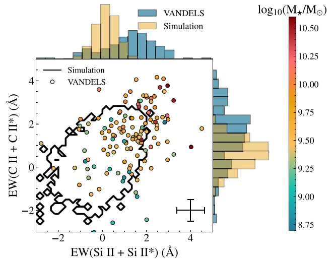
Figure 2. The comparison of the EW(C II \lambda 1334 + C II* \lambda 1335 ) and EW(Si II \lambda 1260 + Si II* \lambda 1265 ) in the simulation (black contour) and in the VANDELS observations (circles). The VANDELS points are color-coded by their stellar mass (the virtual galaxy has M_* within \sim 10^9 - 10^{10.5} M_\odot ), and we show in the bottom right the typical uncertainty on the measurements. The black contour includes the entire range of the mock spectra measurements. The VANDELS galaxy sample exhibits a marginally wider range of EW values, featuring notably larger values in comparison to the simulation.
