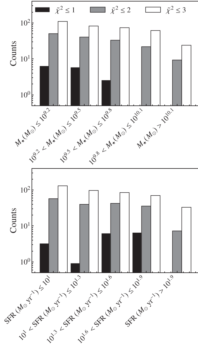
Figure 5. Top: histogram presenting the average number of mock spectra with \tilde{\chi}^2 < 1 (black), \tilde{\chi}^2 < 2 (gray), and \tilde{\chi}^2 < 3 (white) per observed galaxy, in bins of stellar mass. The most massive VANDELS galaxies ( \sim > 10^{10} ) are not well replicated by the mock spectra for our virtual galaxy. Bottom: same, but for the SFR.
