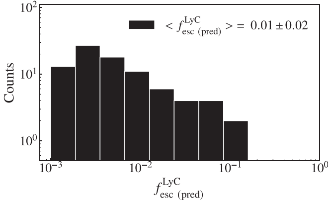
Figure 7. The distribution of f_{\text{esc}}^{\text{LyC}} for the VANDELS sample analyzed in this work. The f_{\text{esc}}^{\text{LyC}} is determined by taking the average f_{\text{esc}}^{\text{LyC}} value across the 30 best mock spectra for each of the 93 selected VANDELS objects. The average f_{\text{esc}}^{\text{LyC}} for this sample is 0.01 \pm 0.02 .
