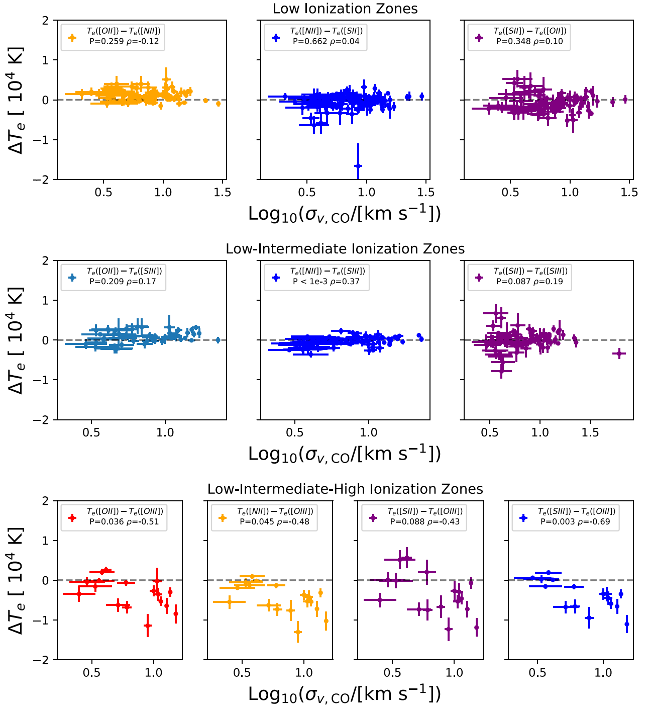
Figure 17. Electron temperature differences compared to the CO velocity dispersion, \sigma_{v,\text{CO}} . The order of the panels follows that in Figure 12. We observe a weak correlation between \Delta(T_{e,[N\ II]}, T_{e,[S\ III]}) . Although insignificant according to their p -values, we also observe that highest T_{e,[O\ III]} values are associated with the highest \sigma_{v,\text{CO}} .
