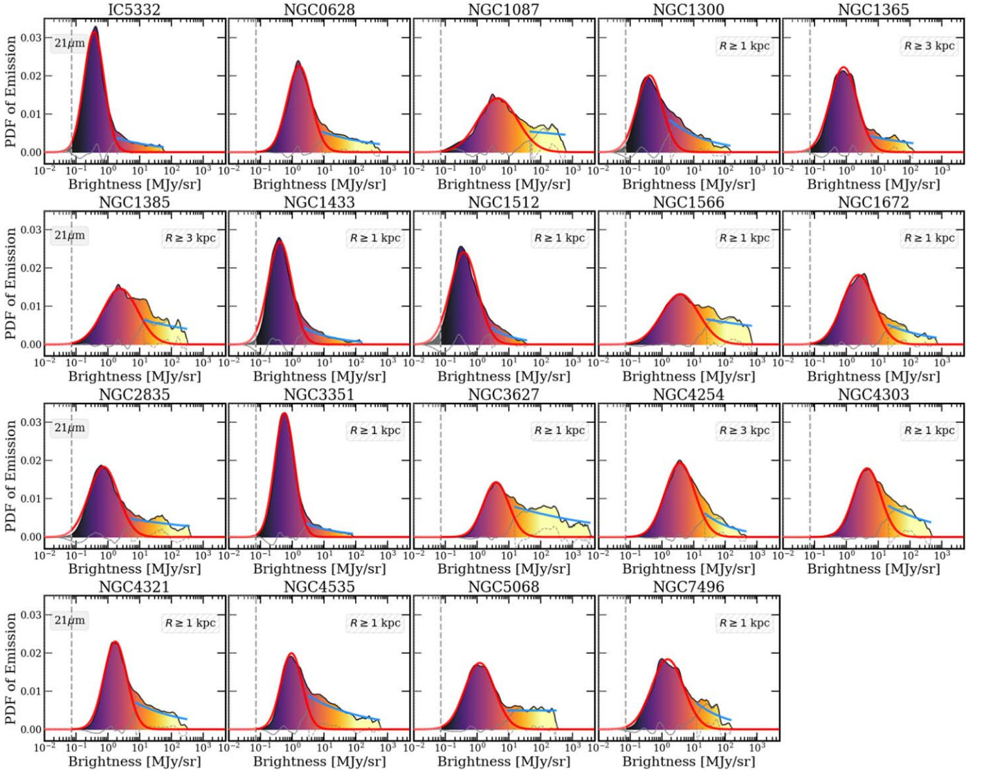
Figure 4. The PDFs of the galactic disk (in black) for our full sample at 21\ \mu\text{m} . Vertical dashed lines show the rms noise levels for 21\ \mu\text{m} at 0.85'' . The PDFs at each filter show an overall distribution well fit by a lognormal (red) at lower intensity (residuals in gray), with high-intensity residuals (dashed gray) that are well fit by a power law (blue).
