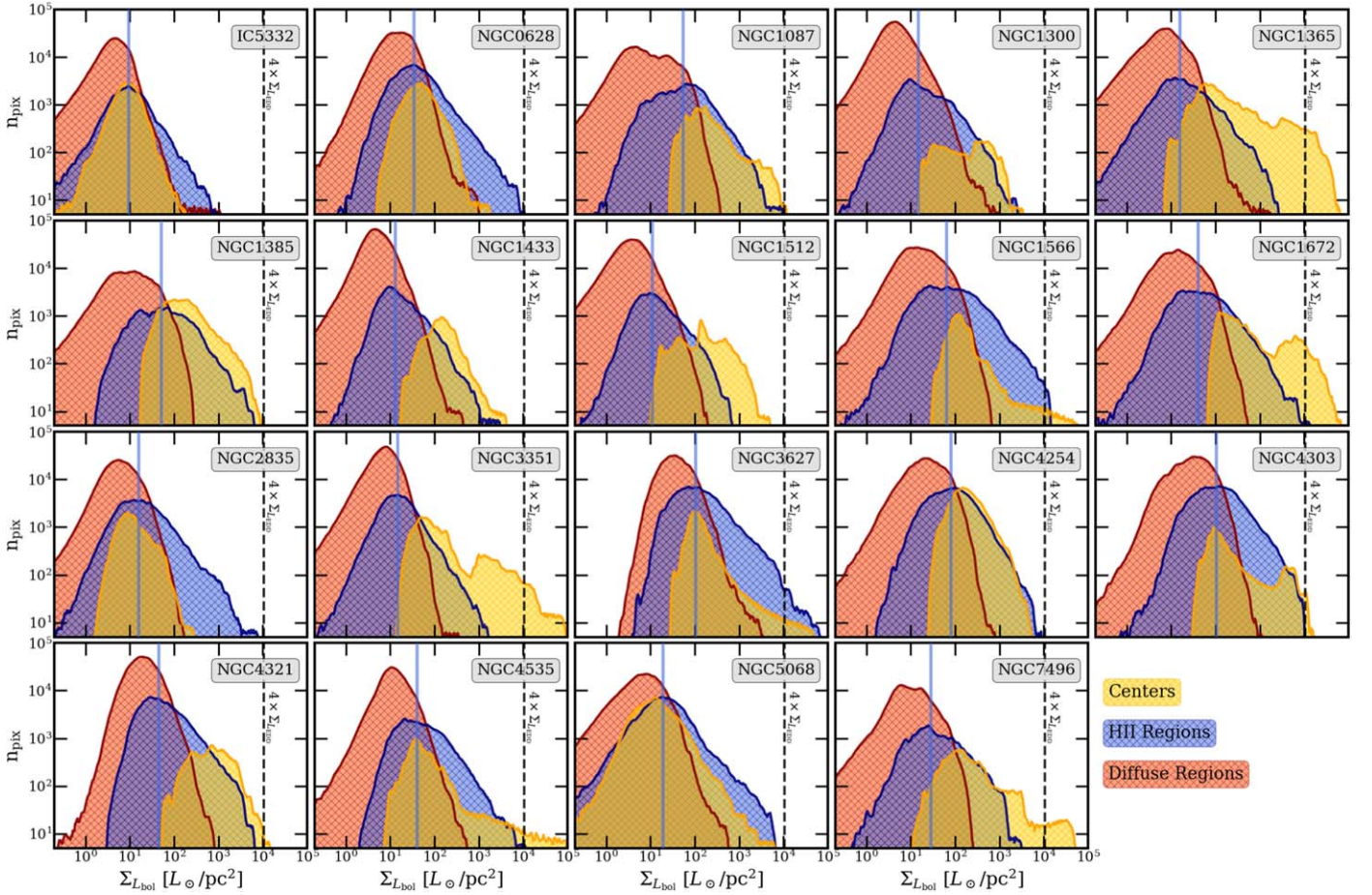
Figure 15. Histograms of pixel-wise bolometric luminosity surface density \Sigma_{L_{\text{bol}}} from the center (yellow), diffuse component (red), and H II regions (blue) for each of our targets. The median \Sigma_{L_{\text{bol}}} for H II regions (vertical blue line) remains roughly consistent between targets. The vertical dashed line shows the estimated Eddington luminosity surface density in star-forming regions, scaled from \mathcal{F}_{L_{\text{bol}}} to \Sigma_{L_{\text{bol}}} units for direct comparison.
