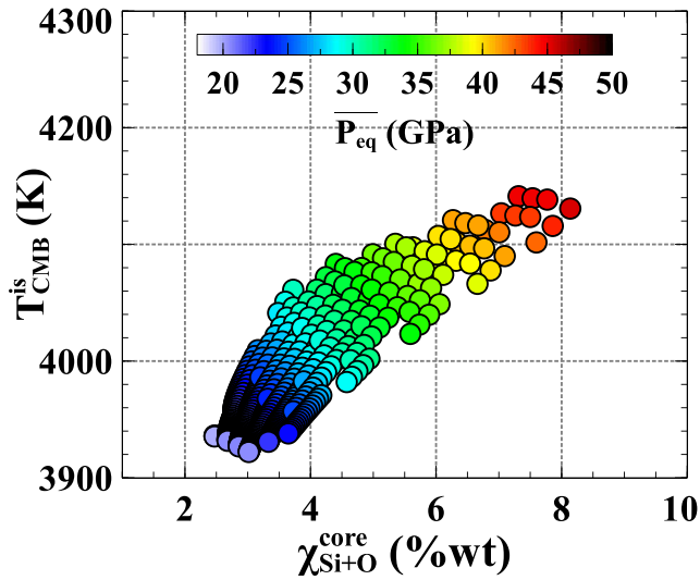
Figure 1. Summary of the results from Clesi & Deguen (2023), showing the correlation between the isentropic temperature at the CMB at the end of accretion ( y -axis), light elements concentration in the core (here Si and O, x -axis) and mean value of equilibrium pressure ( P_{\text{eq}} , colour scale). The temperatures obtained here are obtained with the Grüneisen parameter calculated with Al'Tshuler formalism, with \gamma_0 = 1.875 and \gamma_\infty = 1.305 . The points plotted here are the models matching the compositional constraints defined in Clesi & Deguen (2023).
