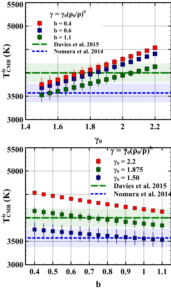
Figure 5. Top panel: effect of \gamma_0 on T_{\text{CMB}}^{\text{is}} for different values of b . Red squares: b = 0.4 . Dark blue squares: b = 0.6 . Dark green squares: b = 1.1 . Bottom panel: effect of b on T_{\text{CMB}}^{\text{is}} for different values of \gamma_0 . Red squares: \gamma_0 = 2.2 . Dark green squares: \gamma_0 = 1.875 . Dark blue squares: \gamma_0 = 1.5 . T_{\text{CMB}}^{\text{is}} is calculated from eqs (8) and (11). For comparison, we also show the estimates of present-day CMB temperature from Nomura et al. (2014) (dotted blue line, lower estimate) and the review of Davies et al. (2015) (dashed green line).
