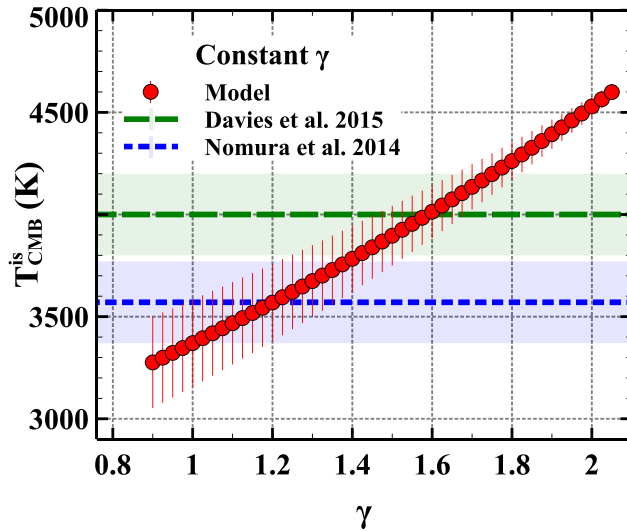
Figure 4. Variation of the mean T_{\text{CMB}}^{\text{is}} determined by eqs (8) and (9) as a function of \gamma . The error bars are the 2\sigma variation on the subset of core formation models used in this study. For comparison the estimates of current CMB temperature from Nomura et al. (2014) (dotted blue line) and Davies et al. (2015) (dashed green line) are also shown.
