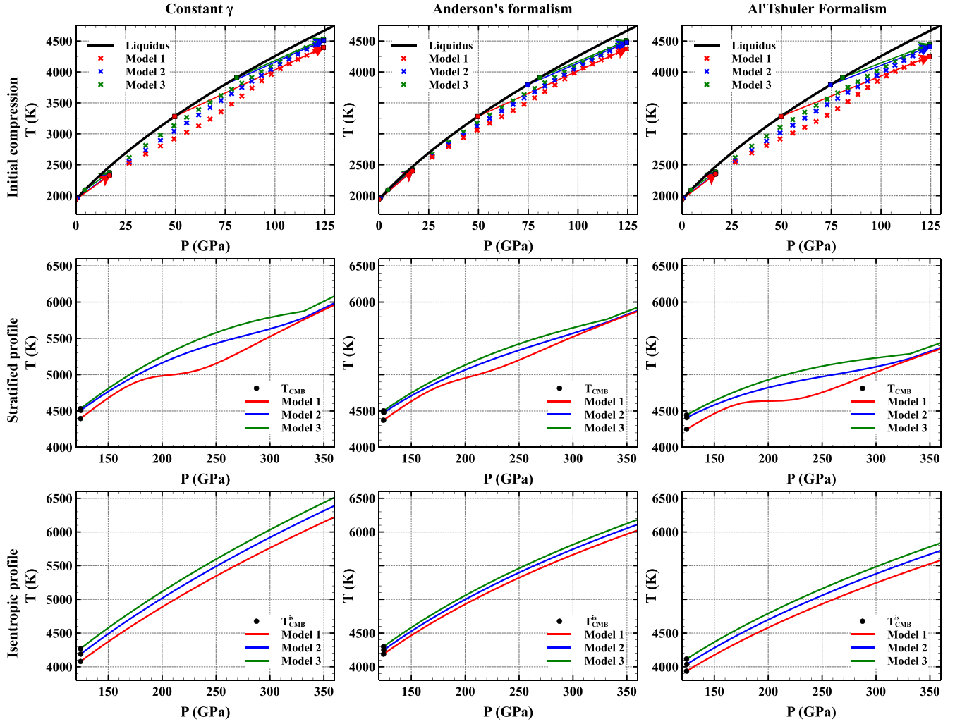
Figure 2. Description of three steps of the model for different formalisms of the Grüneisen parameter tested in this study. Left-hand column: constant \gamma = 1.7 . Middle column: Anderson's power law, with \gamma_0 = 2.05 and b = 0.6 . Right-hand column: Al'Tshuler formalism with \gamma_0 = 1.305 and \gamma_\infty = 1.875 . Each row represents one of the steps of the scenario described in Section 2.1. Top row: initial compression between the bottom of the magma ocean and the growing core-mantle boundary (step (i) and part of step (ii) in the text), with the liquidus curve in black and the adiabat of the first and last steps of the model shown by the arrows. The cross symbols represent the P - T conditions of the metal reaching the CMB at each step of accretion, before the core is fully formed. The arrows show the changes in P - T conditions undergone by the metal through the crystallized part of the mantle in the first step of accretion (round markers) and last step of accretion (square markers). Middle row: temperature profile of the core when stratified and after compression of the metal due to the growth of the core (step (ii) and step (iii) in the text). Bottom row: temperature profile in the core after mixing to an isentropic state (step (iv) in the text). The black dots mark the temperature at the CMB. A similar figure with more details on the model steps can be found at Clesi & Deguen (2023). Red curves: Model 1, obtained for the f_c = 0.6 , a_p = 0.4 and \lambda = 5 , with \bar{P}_{\text{eq}} = 19.7 GPa and \chi_{\text{Si}+\text{O}}^{\text{core}} = 2.47 per cent. Blue curves: Model 2, obtained for the f_c = 0.85 , a_p = 0.6 and \lambda = 1 , with \bar{P}_{\text{eq}} = 34.1 GPa and \chi_{\text{Si}+\text{O}}^{\text{core}} = 5.24 per cent. Green curves: Model 3, obtained for the f_c = 1 , a_p = 0.65 and \lambda = 0.4 , with \bar{P}_{\text{eq}} = 43.9 GPa and \chi_{\text{Si}+\text{O}}^{\text{core}} = 7.86 per cent.
