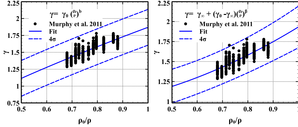
Figure 3. Results of the fit from the data of Murphy et al. (2011) with the formalism of Anderson (1967) (left-hand panel) and Al'Tshuler et al. (1987) (right-hand panel). The data from Murphy et al. (2011) have been bootstrapped to account for the error bar by randomly distributing 20 values for each point following a Gaussian distribution, thus allowing the fit to be made on \sim 200 points instead of 10.
