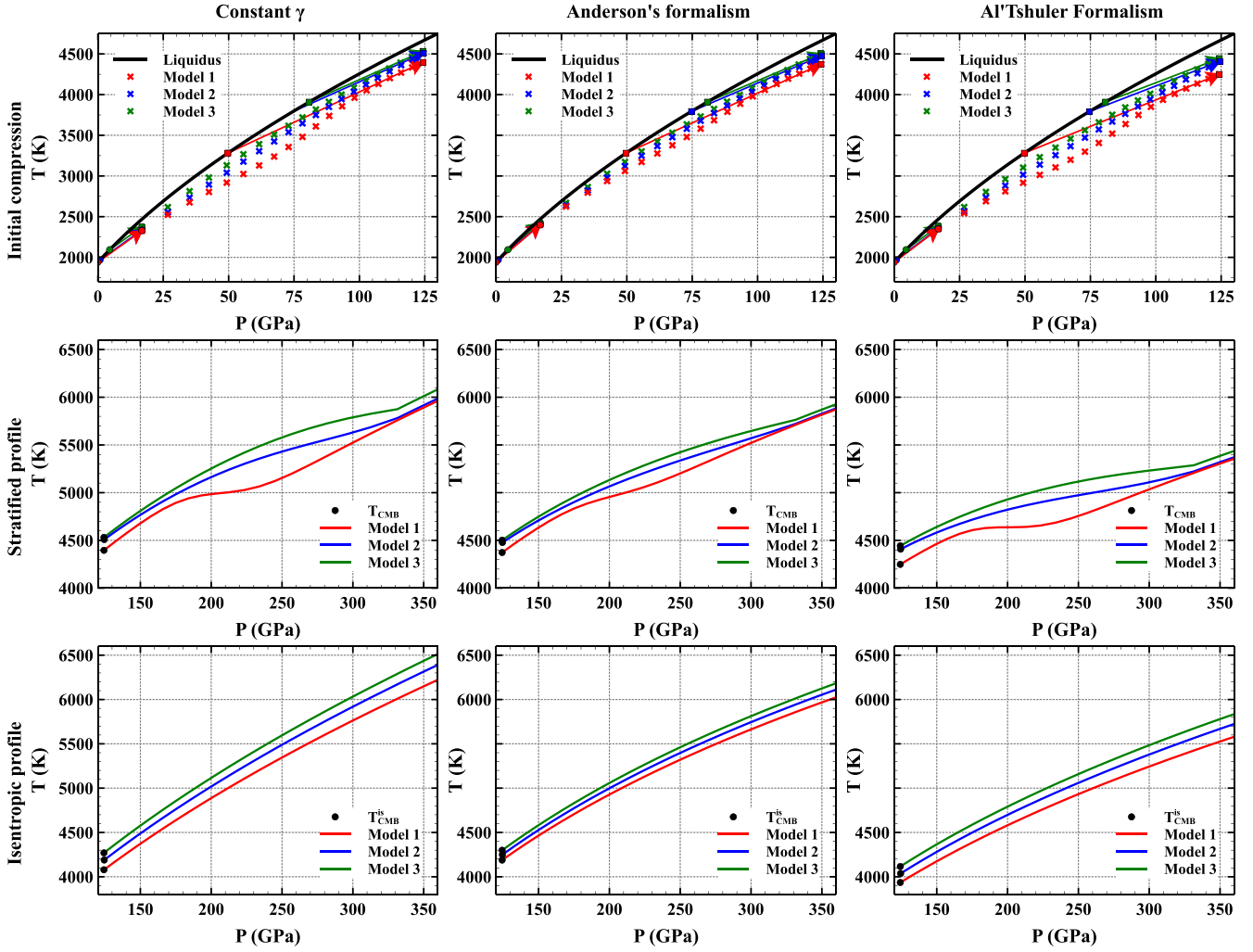
Figure 2. Description of three steps of the model for different formalisms of the Grüneisen parameter tested in this study. Left-hand column: constant \gamma = 1.7 . Middle column: Anderson's power law, with \gamma_0 = 2.05 and b = 0.6 . Right-hand column: Al'Tshuler formalism with \gamma_0 = 1.305 and \gamma_\infty = 1.875 . Each row represents one of the steps of the scenario described in Section 2.1. Top row: initial compression between the bottom of the magma ocean and the growing core-mantle boundary (step (i) and part of step (ii) in the text), with the liquidus curve in black and the adiabat of the first and last steps of the model shown by the arrows. The cross symbols represent the P - T conditions of the metal reaching the CMB at each step of accretion, before the core is fully formed. The arrows show the changes in P - T conditions undergone by the metal through the crystallized part of the mantle in the first step of accretion (round markers) and last step of accretion (square markers). Middle row: temperature profile of the core when stratified and after compression of the metal due to the growth of the core (step (ii) and step (iii) in the text). Bottom row: temperature profile in the core after mixing to an isentropic state (step (iv) in the text). The black dots mark the temperature at the CMB. A similar figure with more details on the model steps can be found at Clesi & Deguen (2023). Red curves: Model 1, obtained for the f_c = 0.6 , a_p = 0.4 and \lambda = 5 , with \bar{P}_{\text{eq}} = 19.7 GPa and \chi_{\text{Si}+\text{O}}^{\text{core}} = 2.47 per cent. Blue curves: Model 2, obtained for the f_c = 0.85 , a_p = 0.6 and \lambda = 1 , with \bar{P}_{\text{eq}} = 34.1 GPa and \chi_{\text{Si}+\text{O}}^{\text{core}} = 5.24 per cent. Green curves: Model 3, obtained for the f_c = 1 , a_p = 0.65 and \lambda = 0.4 , with \bar{P}_{\text{eq}} = 43.9 GPa and \chi_{\text{Si}+\text{O}}^{\text{core}} = 7.86 per cent.
