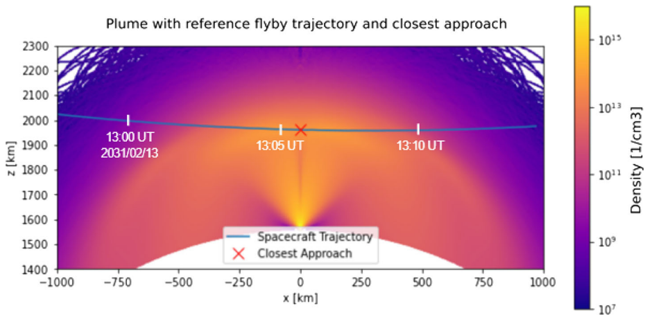
Fig. 19 JUICE trajectory through a model 100 kg/s collisional plume, with closest approach at an altitude of 400 km. The time that JUICE encounters the plume ( \sim 10 mins) well exceeds the PEP-NIM integration time (5 s), therefore the plume structure (e.g. the canopy shock) can be discerned, allowing to empirically constrain plume models and study internal plume physics. [Reproduced from Dayton-Oxland et al. 2023]
