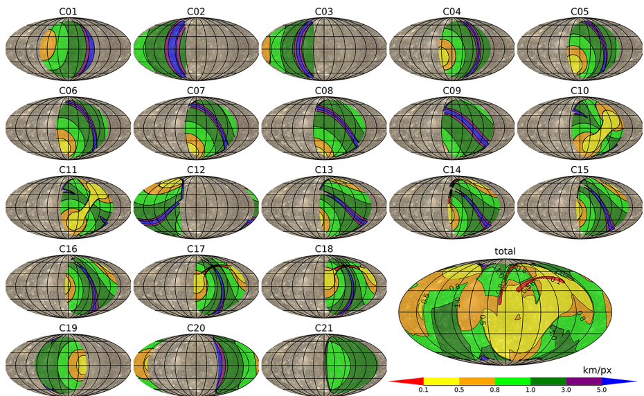
Fig. 11 Plots of maximum diurnal coverage obtainable by MAJIS during the Callisto flybys, labelled C01 to C21, assuming a recently predicted JUICE mission profile (CRcMA 5.0). Solar incidence angle is imposed <75^\circ and viewing geometry in near-nadir direction (within 15^\circ from nadir). The colour scale in each plot represents the best spatial resolution achievable by MAJIS. The larger map in the lower-right panel displays the potential coverage achievable by merging the coverage of all flybys with the best spatial resolution
