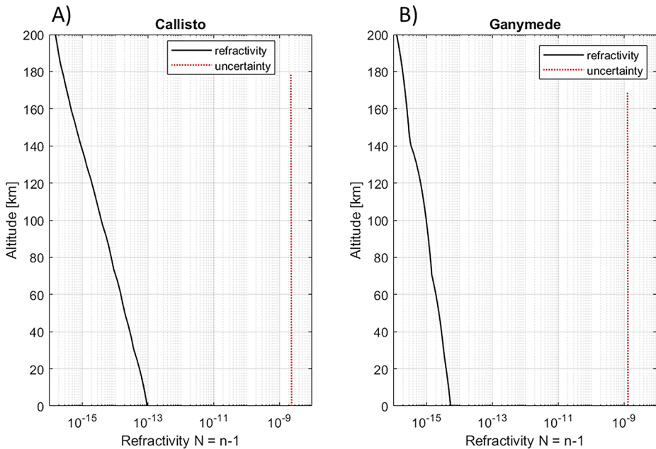
Fig. 16 Predicted refractivity height profile of Callisto (panel A) and Ganymede (panel B) (black line), compared to the expected measurement's uncertainty (red dotted line) of the 3GM radio science experiment (figure courtesy of A. Caruso)
