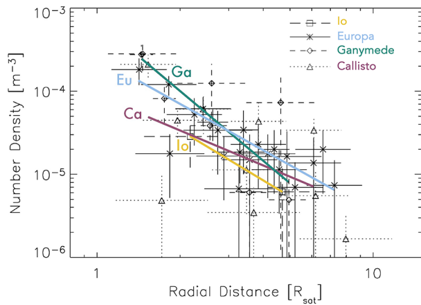
Fig. 14 Number density of dust as a function of radial distance from the centre of Ganymede, Europa, Callisto, and Io, measured by the Galileo Dust Detector System. Adapted from Krüger et al. (2003)
