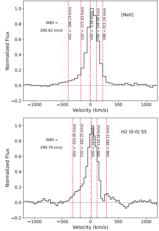
Fig. E.1. Non-parametric analysis of two nuclear line profiles: [Ne II] (top panel) and H 2 S(5) (bottom panel). The derived velocities (see text for details) are marked with red vertical lines. The gray lines indicate the limits of the emission line defined as fluxes above two times the standard deviation of the (zero) continuum.
