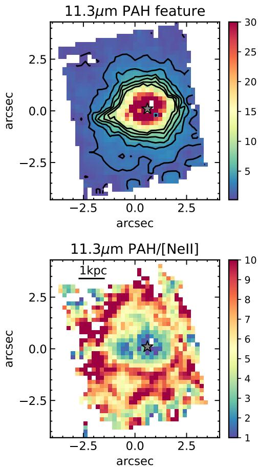
Fig. 7. Maps of the intensity of the 11.3 \mu\text{m} PAH feature (top) in units of 10^{-16} \text{erg cm}^{-2} \text{s}^{-1} and the 11.3 \mu\text{m} PAH to [Ne II] line ratio (bottom). The FoV and symbols are as in Fig. 6. The maps and contours are in a linear scale.
