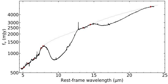
Fig. 2. MRS nuclear spectrum (solid black line) of Mrk 231. It was extracted with a 1'' -radius aperture and covers the rest-frame \sim 4.7 – 23.5 \mu\text{m} spectral range. We applied the residual fringing correction to the extracted 1D spectra of each of the sub-channels. The dotted line is the fitted continuum using a cubic spline function and the red dots are the anchor points selected for the fit.
