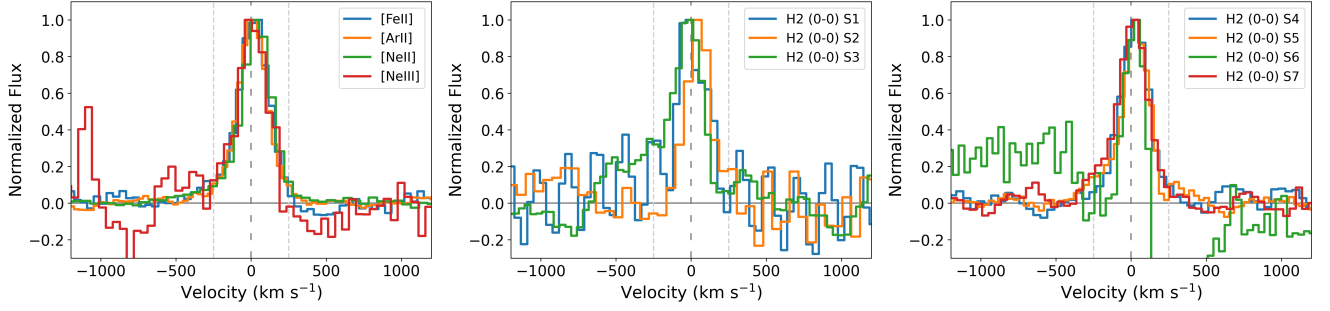
Fig. 12. Line profiles from the nuclear region ( r = 1'' aperture). Left panel: fine-structure lines, and middle and right panels: H 2 S(7) to S(4) and S(3) to S(1) transitions, respectively. The 0 km s -1 value corresponds to the adopted z = 0.004217 . Note that the red part of the H 2 S(6) line profile (green line, middle panel) is inside one of the H 2 O molecular absorptions. We did not apply the 1D residual fringe correction.
