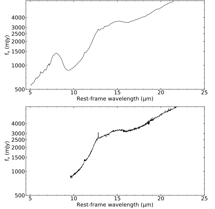
Fig. B.1. Spitzer /IRS spectra of Mrk 231. Those obtained with the low-resolution modules SL and LL are in the top panel and those of the high-resolution modules SH and LH in the bottom. Wavelength and flux density ranges are as in Fig. 2.
