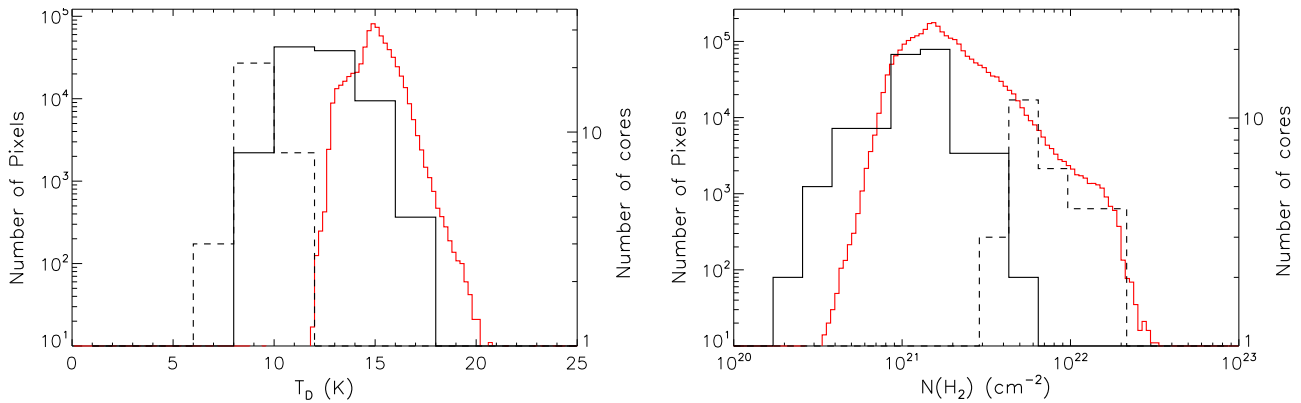
Figure 14. Histograms of ( left ) fitted SED temperatures and ( right ) core background-subtracted peak N(\text{H}_2) column densities at the 500\ \mu\text{m} resolution. The right-hand axis and the black curve on each plot show the histogram for unbound starless cores (solid line) and prestellar cores (dashed line). The left-hand axis and the red curve on each plot show the histogram of all valid pixel values in the map from Fig. 2.
