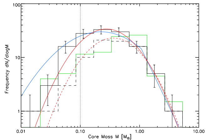
Figure 18. The combined mass function for the L1495 and TMC1 regions. The solid black line shows all prestellar cores, the dashed black line shows robust prestellar cores. The red curve shows a lognormal fit to the prestellar core distribution above the completeness limit of this paper ( 0.1 M_{\odot} , shown by the vertical dotted black line). The blue curve shows a scaled initial mass function (IMF) from Chabrier (2003) and the green curve shows the Taurus IMF derived by Luhman et al. (2009).
