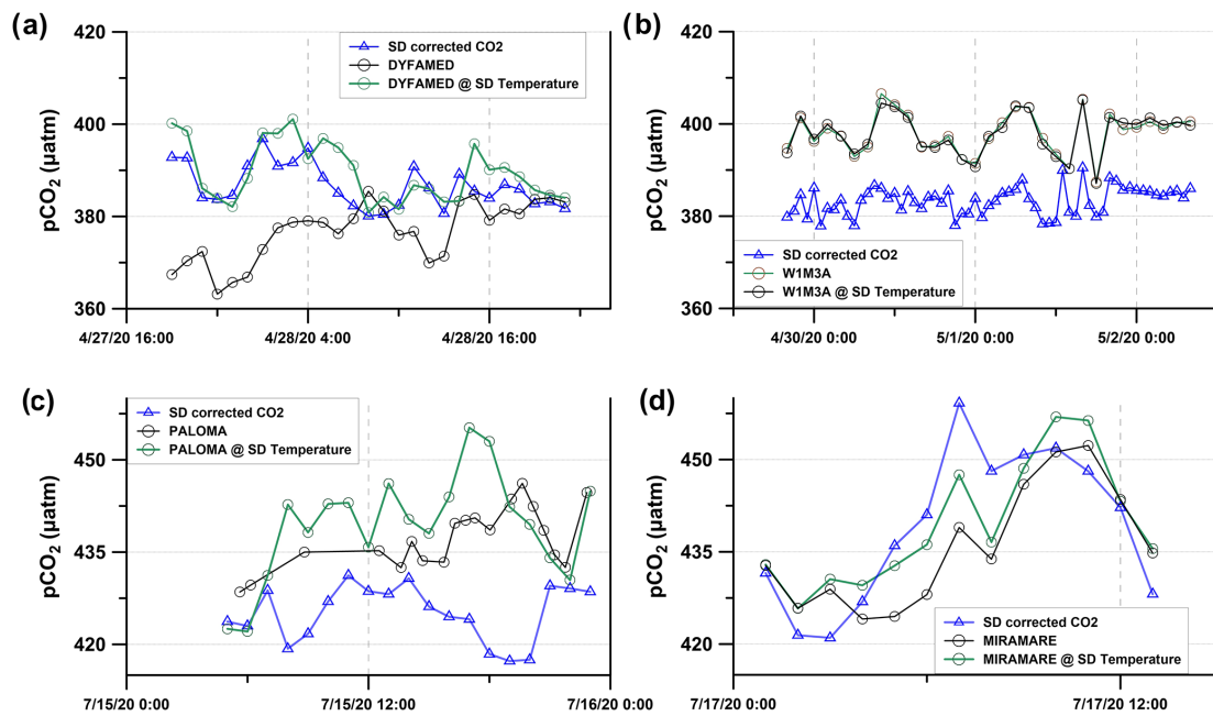
Figure 10. Comparison between p\text{CO}_2 measured by the SD 1030 (blue) and at the fixed ocean stations (black and green): the fixed-ocean-station p\text{CO}_2 measured at in situ depth and temperature (black) and the fixed-ocean-station p\text{CO}_2 normalised to surface temperature (green). (a) DYFAMED fixed station, (b) WIM3A fixed station, (c) PALOMA fixed station, and (d) MIRAMARE fixed station.
