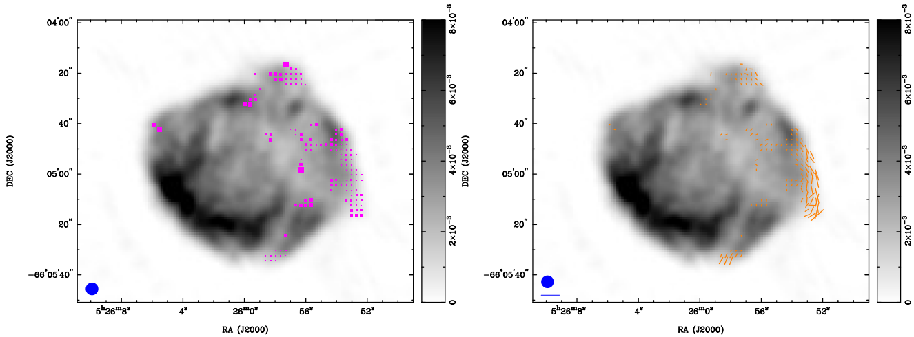
Figure 7. The rotation measure map (left) of N 49 overlaid on 5.5 GHz image. The pink boxes represent RM values estimated from the position angles associated with linear polarisation. The maximum value of RM is \sim 591 \text{ rad m}^{-2} . The blue ellipse in the lower left corner represents the synthesised beam width of 5'' \times 5'' . The image on the right shows magnetic field vectors overlaying the 5.5 GHz radio image.
