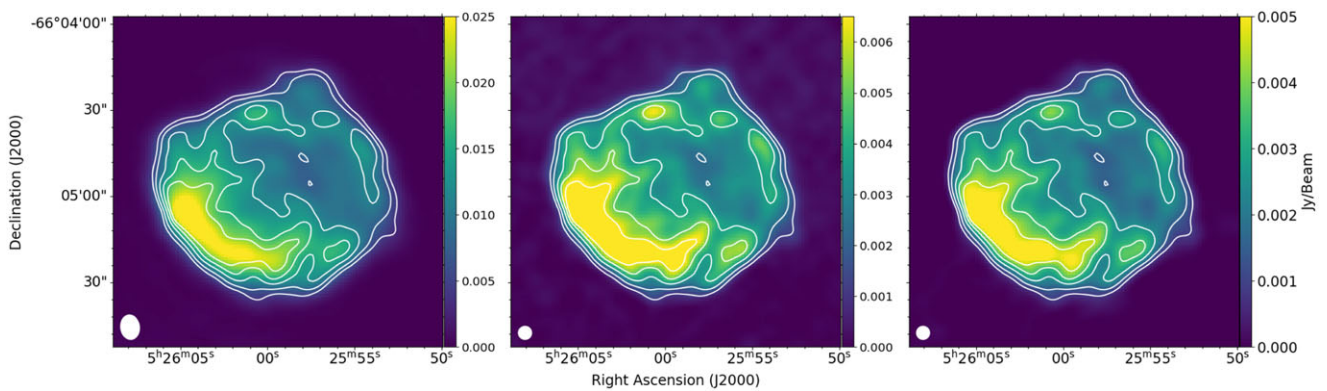
Figure 3. Pre-CABB update radio continuum images of SNR N 49. 4.79 GHz contour levels overlaid on each of the 3 images are 0.85, 1.5, 2.5, 3.5, and 4.5 mJy beam -1 . Left: 2.4 GHz image with a resolution (beam size) of 8.9'' × 6.6''. Middle: 4.79 GHz image with a resolution (beam size) of 5'' × 5''. Right: 8.64 GHz image with a resolution (beam size) of 5'' × 5''. White circles in the lower left corner scale the synthesised beam.
