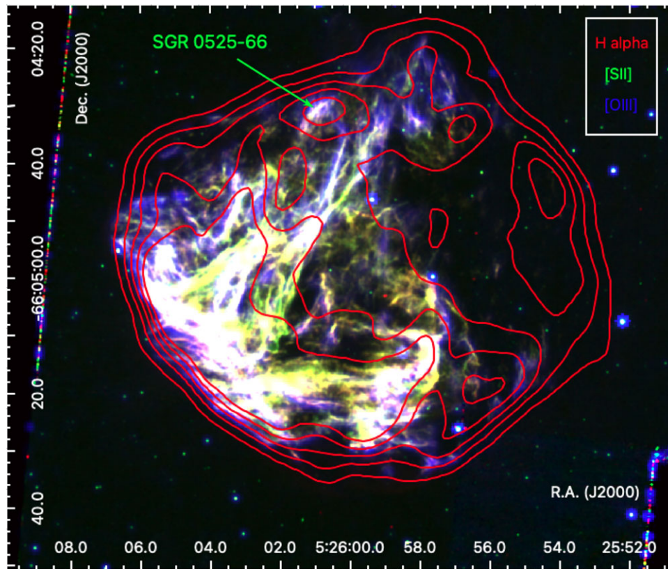
Figure 9. The HST optical image of N 49 as described in Bilikova et al. (2007) (RGB = H \alpha (red), [S ii] (green), and [O iii] (blue) overlaid with 5.5 GHz radio contours (0.25, 1.4, 2.6, 3.8, 5 and 5 mJy beam ^{-1} ).
