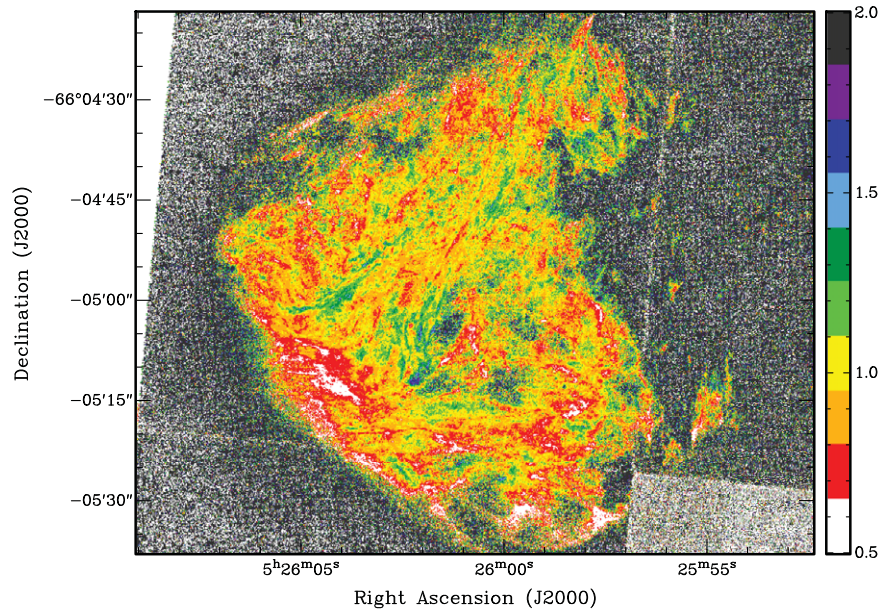
Figure 10. The [S ii]/H \alpha ratio map indicates the bright filaments and extent of emission.
