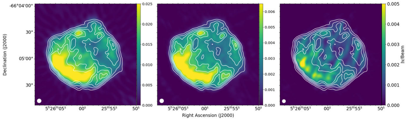
Figure 2. CABB radio continuum images of SNR N 49. 5.5 GHz contour levels overlaid on each of the 3 images are 1, 2, 3, 4, and 5 mJy beam -1 . Left: 2.1 GHz image with a resolution (beam size) of 4'' × 4'' Middle: 5.5 GHz image with a resolution (beam size) of 5'' × 5'' Right: 9 GHz image with a resolution (beam size) of 4'' × 4''. White circles in the lower left corner scale the synthesised beam.
