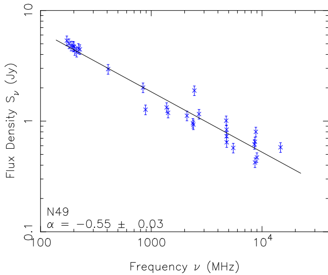
Figure 8. Radio continuum spectrum of N 49 using MWA, ASKAP, and ATCA data (Table 4). The black solid line shows a linear least squares fit in logarithmic space, giving a spectral index of \alpha = -0.55 \pm 0.03 . The relative errors (assumed to be 10%) are shown as vertical bars.
