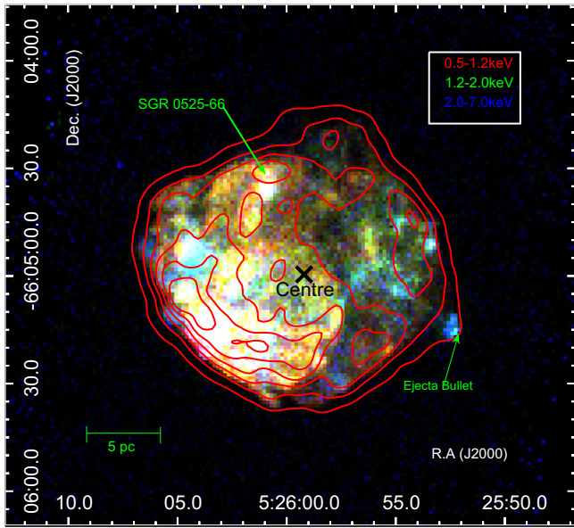
Figure 4. An X-ray three-colour image of N 49 that shows our new Radio data superimposed as contours. Red represents the energy band 0.5–1.2 keV (soft), green corresponds to the energy band 1.2–2.0 keV (Medium) and blue represents the energy band 2.0–7.0 keV (hard). This X-ray image is overlaid with 5.5 GHz radio contours at 0.25, 1.4, 2.6, 3.8, and 5 mJy beam -1 . The distance between SNR centre to the ‘bullet’ feature is used to estimate the upper and lower angular displacement values as explained in Table 3.
