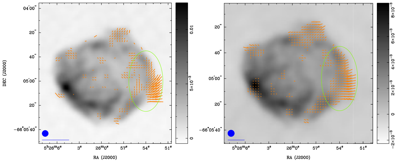
Figure 6. Fractional polarisation vectors overlaid on their corresponding ATCA intensity images. The image on the left is at 4.79 GHz (pre-CABB). large green ellipse in these images indicates an enhanced polarisation region around the proposed ‘bullet ejecta’ or bow-shock PWN. The image on the right is at 8.64 GHz (pre-CABB). The blue circle in the lower left corner of this image represents the synthesised beam width of 5'' \times 5'' and the blue line below, a fractional polarisation vector of 100%.
