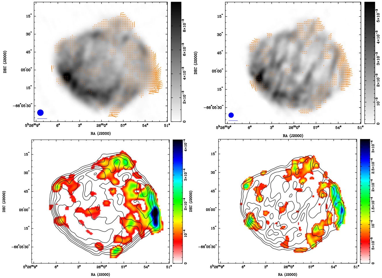
Figure 5. The polarisation map of N 49 at 5.5 GHz (left column) and at 9 GHz (right column) where respective fractional polarisation vectors shown on the top images are overlaid on corresponding intensity ATCA images. The blue circles in the lower left corner represent a synthesised beam of 5'' \times 5'' and 4'' \times 4'' , for 5.5 and 9 GHz, respectively. The blue line below the circles represents 100% polarisation. The bar on the right side represents the greyscale intensity gradients for the ATCA images in \text{Jy beam}^{-1} . Polarisation intensity maps at 5.5 GHz (bottom left) and at 9 GHz (bottom right) are shown in the bottom images with radio intensity contour lines overlaid; radio contours are 0.05, 1, 2, 4, and 6 \text{mJy beam}^{-1} for 5.5 and 9 GHz, respectively.
