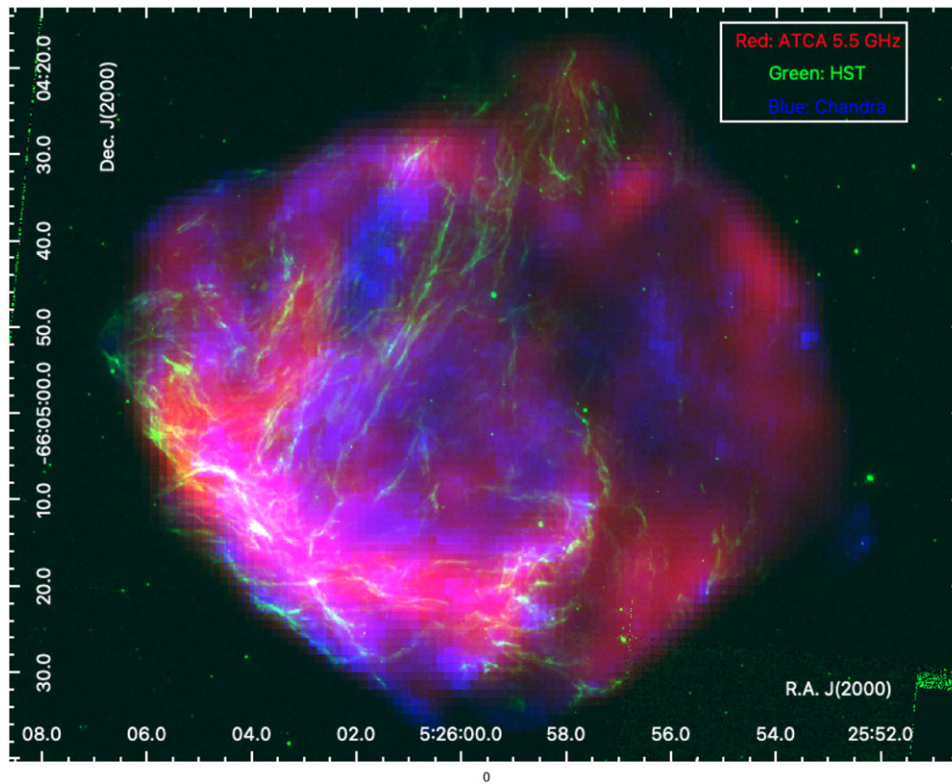
Figure 1. Combined RGB map of N 49 where Red is radio (5.5 GHz ATCA), Green is optical (HST) and Blue is X-ray (Chandra).
