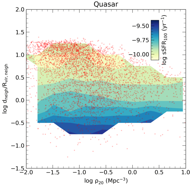
Figure 12. Contours of specific star formation rate ( sSFR_{100} ) in quasar mode in \rho_{20} - d_{\text{neigh}}/R_{\text{vir,neigh}} plane. The red points show the distribution of quasars in the plane. For a given sSFR_{100} value, contours are aligned horizontally, indicating that d_{\text{neigh}}/R_{\text{vir,neigh}} is the dominant quantity in determining SFR in presence of a close neighbor. The high values of sSFR at low neighbors correspond to currently interacting and recent major merger cases respectively.
