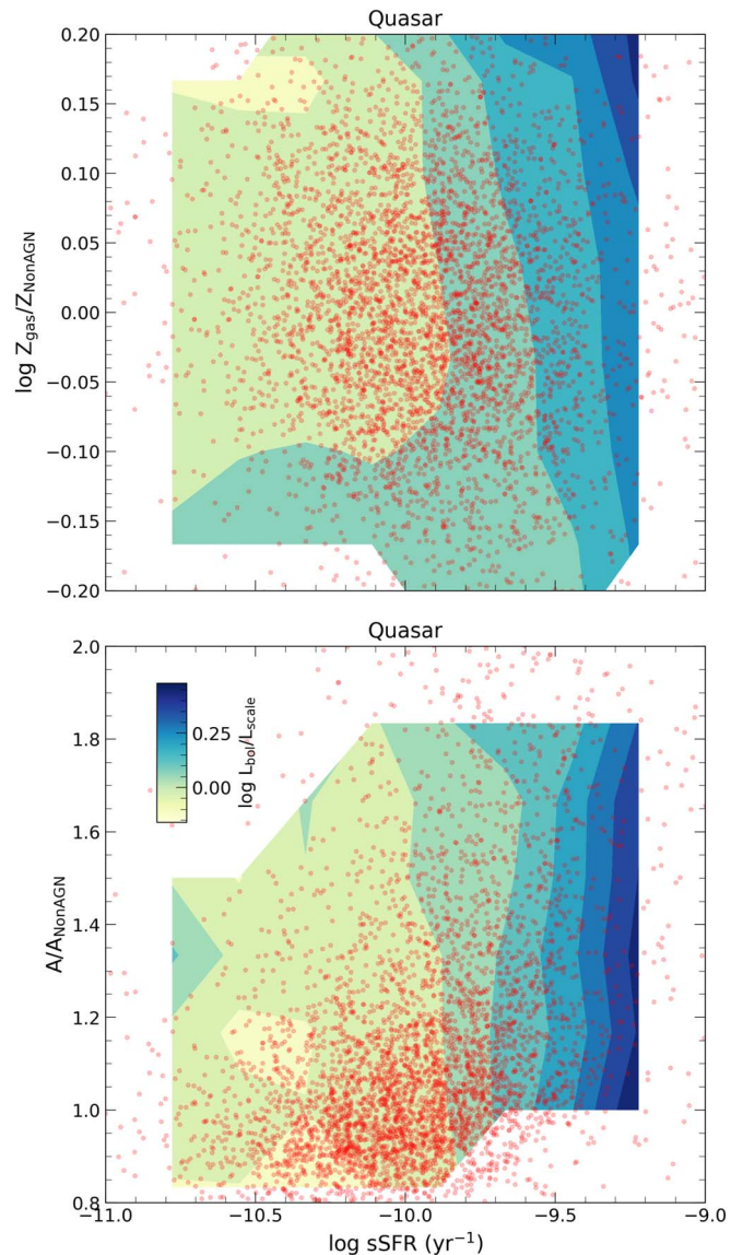
Figure 6. Contours of bolometric luminosity in quasar mode in \text{sSFR}\text{-}A/A_{\text{NonAGN}} plane and \text{sSFR}\text{-}Z_{\text{gas}}/Z_{\text{NonAGN}} plane. The red points show the distribution of quasars in the two planes. For a given value of bolometric luminosity, the contours are aligned vertically. Therefore, the sSFR is the dominant intrinsic property determining the bolometric luminosity of the AGN in quasar mode. Note that, for low sSFR ( <10^{-10}\text{ yr}^{-1} ) and low gas metallicity, the contours are not vertical, and bolometric luminosity changes with the decrease in gas phase metallicity.
