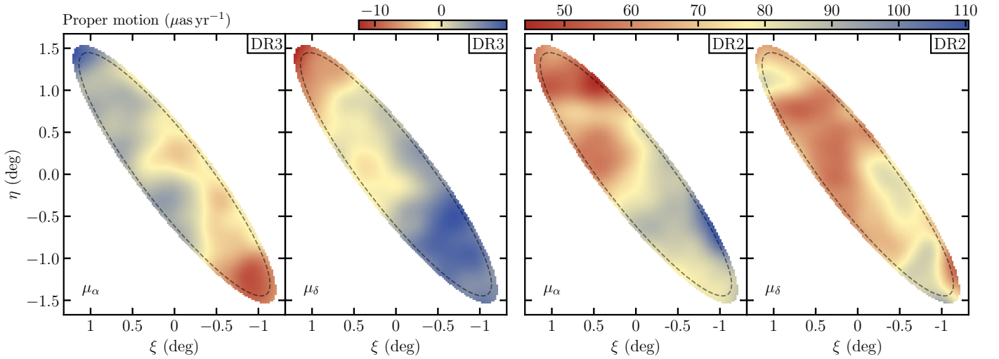
Fig. 2. Zero-point offsets for the Gaia stars' proper motions. Left-hand panels: smoothed maps of the quasar proper motions in the right ascension and the declination directions obtained using Gaia DR3. Right-hand panels: same but using Gaia DR2.
