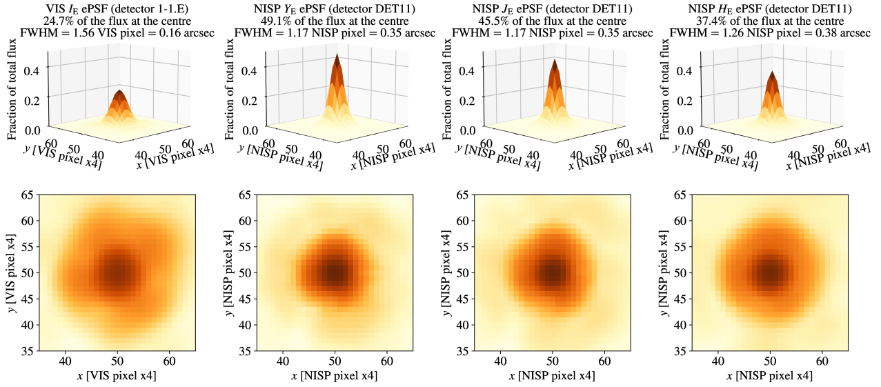
Fig. 3. Overview of the Euclid 's ePSFs modelled in our analysis. The top row shows a 3D representation of our ePSFs for the VIS quadrant 1-1.E and for the NISP detector DET11 in each of the three NISP filters. At the top of each panel, we provide the percentage of flux of the star within the centremost pixel, and the full width at half maximum (FWHM) in pixel and in arcsec. The bottom row contains the 2D view of the ePSFs. The scale is logarithmic and the same in all these four panels.
