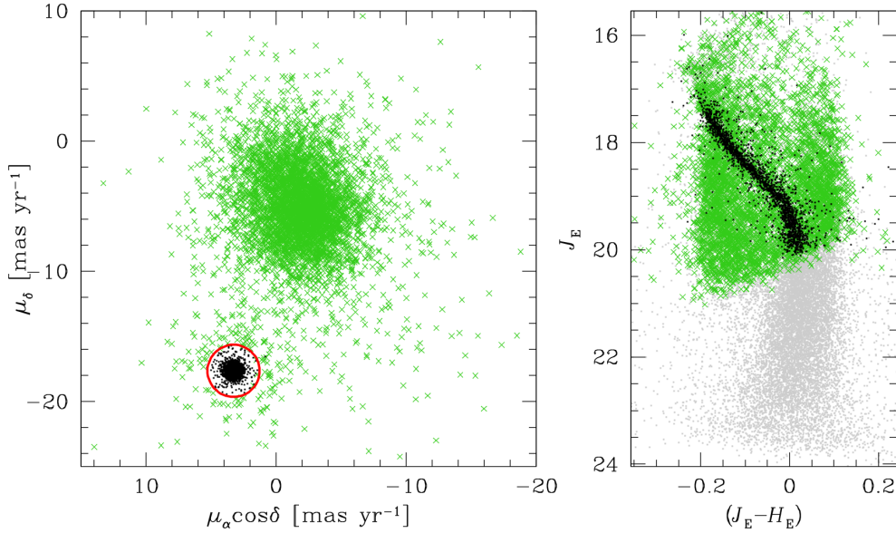
Fig. 12. Overview of the VPD and CMD of stars with E - G PMs. In the VPD on the left, we selected members of NGC 6397 (black points) as those objects having a PM within 2 \text{ mas yr}^{-1} of the bulk motion of the cluster (red circle). All other stars are considered background or foreground field populations and are shown in green. All objects, including those saturated, are shown for completeness. The two groups of stars are then plotted in J_E as a function of (J_E - H_E) on the right. Our PMs are effective in discriminating between the various populations in the field. As a reference, we show in grey all other stars in the catalogue that do not have a PM measurement because they are fainter than the Gaia limit. The main limitation of our investigation is the shallow first-epoch Gaia catalogue used to compute PMs. Only 10% of points are shown for clarity.
