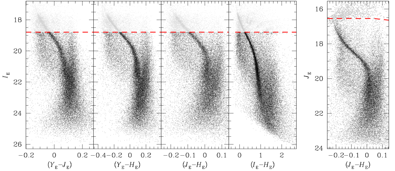
Fig. 10. Collection of CMDs made using our VIS and NISP catalogues. The red dashed lines mark the saturation threshold in each plot. Unsatuated objects are shown in black, while saturated sources are depicted in grey. No quality selections are applied. Only 20% of the points are shown for clarity.
