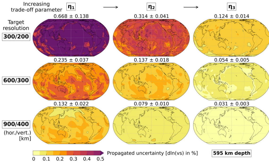
Figure 14. Propagated model uncertainty \sigma_{\hat{m}^{(k)}} at 595 km depth for different target kernel sizes and trade-off parameters. Dashed contour lines are only drawn at the values shown in the colour bar. Values above each map show the global mean \pm standard deviation.
