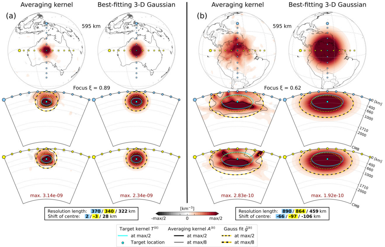
Figure 7. Averaging kernels A^{(k)} and their best-fitting Gaussians \hat{g}^{(k)} using (a) the high-resolution setup ( \eta_1 , T^{(k)} ) with horizontal and vertical extent w_{H/V} = 300/200 km, below Western Australia and (b) the low-resolution setup ( \eta_3 , T^{(k)} ) with w_{H/V} = 900/400 km, below Venezuela. Both target locations and the corresponding lateral cross-sections are at 595 km depth. Vertical cross-sections are marked by blue and yellow dots. Larger dots specify the negative direction for the local coordinate system in which resolution lengths and shifts of the centre are quantified. Additionally, the value for the focus \xi is shown, which serves as a metric for quantifying the appropriateness of \hat{g}^{(k)} (see Section 4.2).
