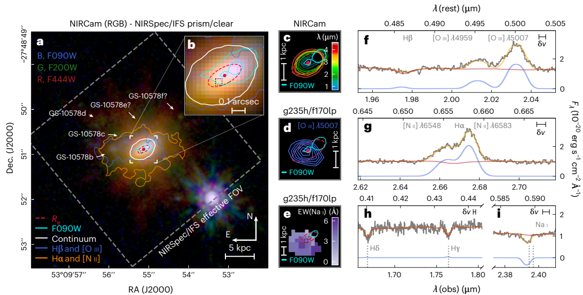
Fig. 1 | Summary of GS-10578 observations. a , NIRCcam false-colour image. The grey dashed square is the field of view of NIRSpec/IFS (with dithering). The solid white contour is a stellar isophote from NIRSpec/IFS prism spectroscopy. The red dashed ellipse is the best-fitting deconvolved model, with semimajor axis 1R_e . The cyan contours are rest-frame UV from NIRCcam F090W, which display the complex morphology, probably due to foreground dust. The orange and blue contours are isosignificance lines for the H\alpha -[N II] and H\beta -[O III] blended lines, from the prism data. Nebular emission is significantly more extended than the stellar light, indicating the ability of mergers and feedback to enrich the circumgalactic medium. b , Detail of the central region of a ; the dashed black square outlines a single NIRSpec spaxel, whose spectrum is reproduced in panels f - i . c , Comparing the model isophote (red dashed ellipse) to NIRCcam isophote morphology, there is a clear wavelength-dependent offset to the north-west. d , Brightest [O III] emission from g235h/f170lp data, showing a slight
