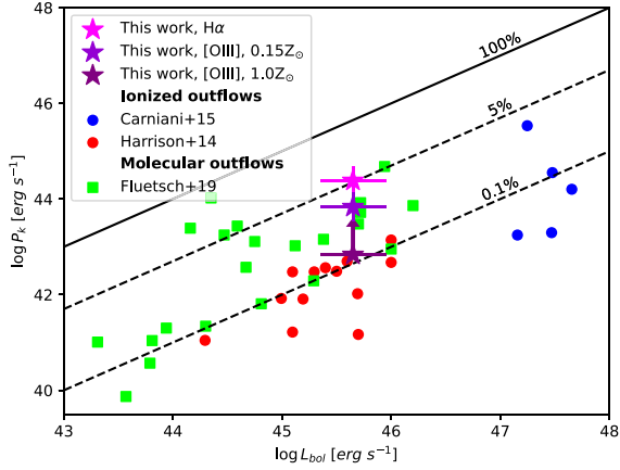
Figure C2. A comparison between the AGN bolometric luminosity, on the x -axis, and outflow kinetic power, on the y -axis, for 28074 QSOs from Carniani et al. (2015), Harrison et al. (2014), and Fluetsch et al. (2019). Molecular outflow data are marked with green squares, while ionized outflows with circles. Our object is indicated by magenta and violet stars for estimates using H\alpha and [O\text{ III}] emission at NLR metallicity, respectively. The lower limit obtained from [O\text{ III}] emission assuming solar metallicity is marked by the purple star. The error bars indicate \sim 0.3 dex systematic uncertainties. The literature data have been adjusted for the factor of 3 discrepancy between assumed geometries. The lines denote constant ratios of 100 per cent, 5 per cent, and 0.1 per cent.
