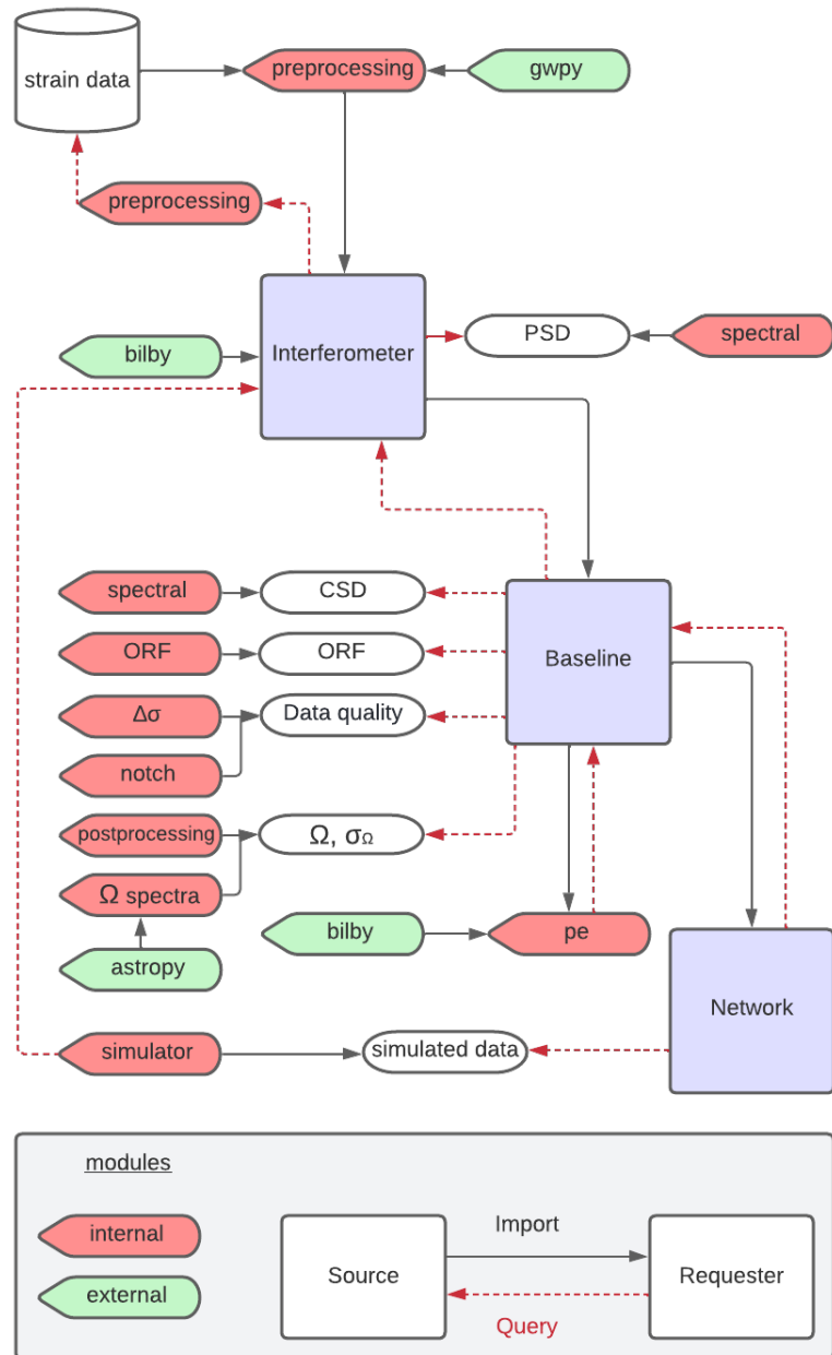
Figure 1: pygwb schema.
