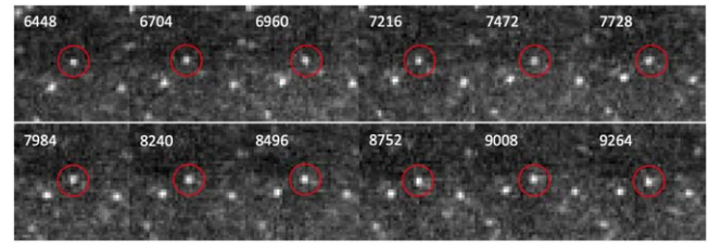
Figure 6. Spitzer/MIPS 24\ \mu\text{m} images of Makemake, with AORKEYs 19176448–19179264 (see Table 1 for the flux densities derived).
