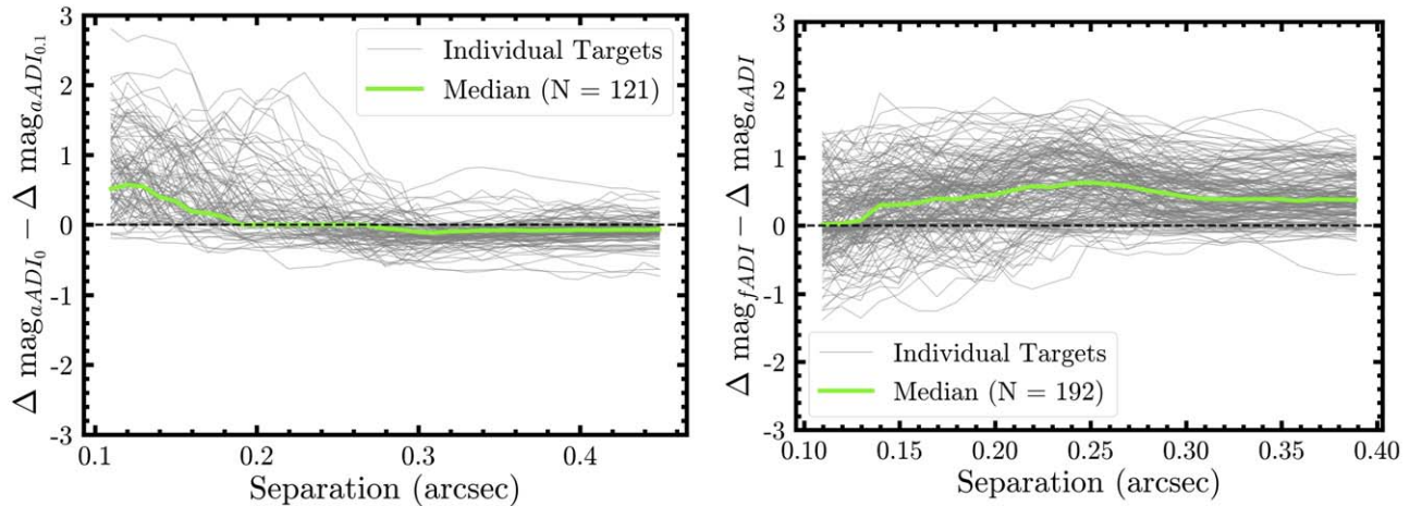
Figure A1. Left: difference in contrast (units of \Delta\text{mag} ) achieved between annular ADI with a rotation gap criterion of 0.1 FWHM ( aADI_{0.1} ) and annular ADI with no rotation gap criterion ( aADI_0 ) as a function of separation (units of arcseconds). A black dashed line marks zero difference and corresponds to both strategies achieving the same sensitivity level. Gray curves correspond to individual targets in the sample and the green curve corresponds to the median computed across all targets. Right: same as the left panel but presenting the difference in contrast achieved between full-frame ADI ( fADI ) and annular ADI ( aADI ). The best-performing strategy varies depending on the individual target.
