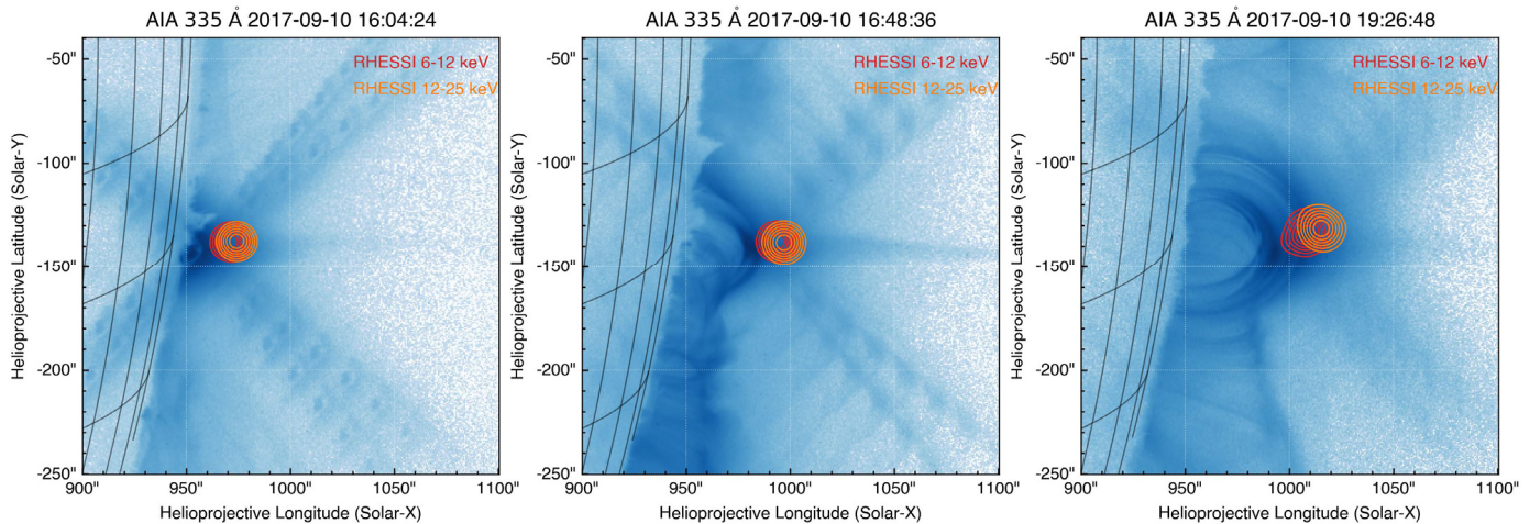
Fig. 5. RHESSI contours of the 6–12 keV (red) and 12–25 keV (orange) source overplotted on 335 Å images at three different times of the event. AIA 335 Å is formed at \log T \sim 6.4 K, similar to the formation temperature of our EIS composition diagnostic pairs. The RHESSI images here were made using the CLEAN reconstruction algorithm with detectors 3, 6, and 8.
