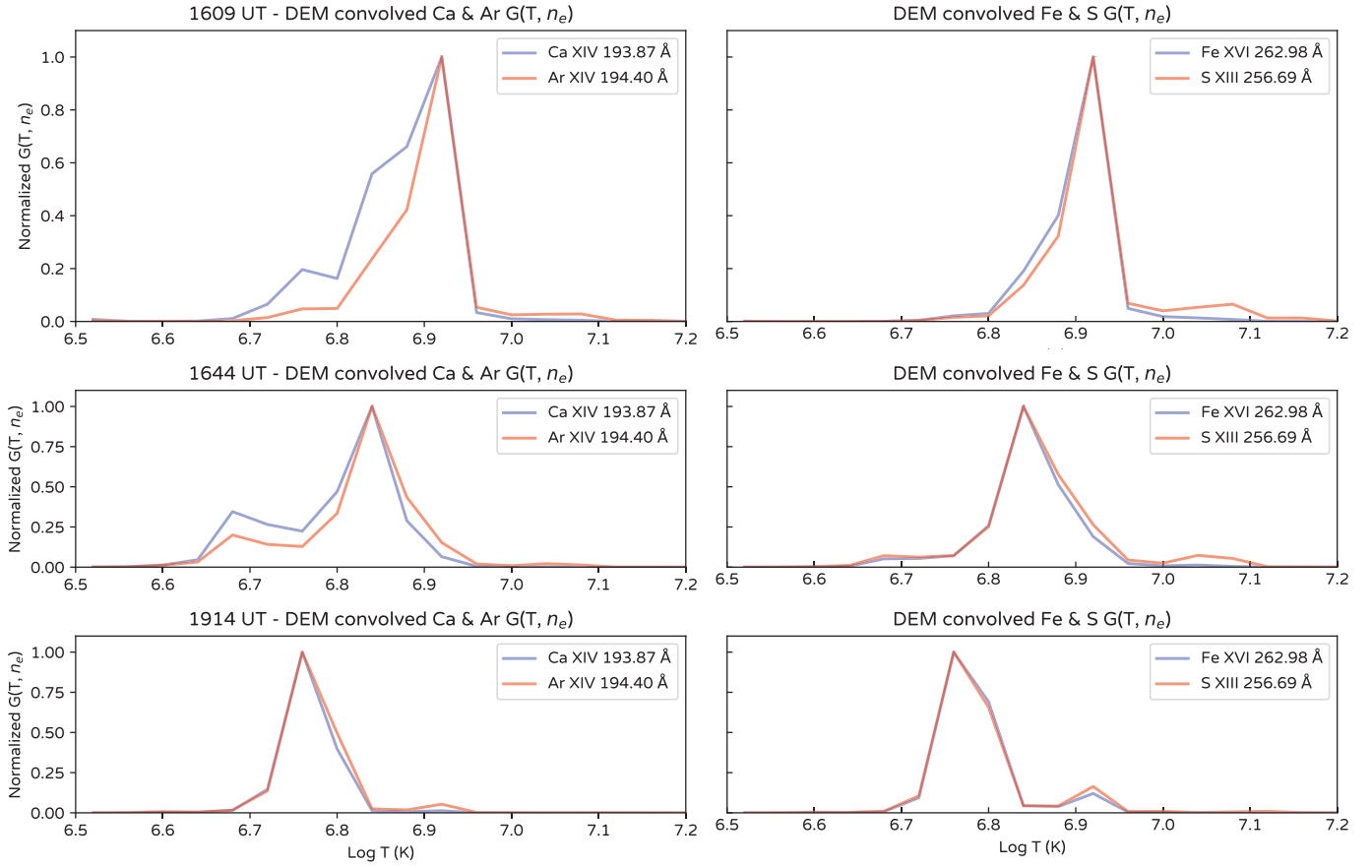
Fig. B.1. Log normalized contribution functions, G(T, n_e) of the Ca XIV 193.87 Å and Ar XIV 194.40 Å (left column), and the Fe XVI 262.98 Å/S XIII 256.69 Å (right column) composition diagnostic pair convolved with the DEM for the flaring looptop at 16:09 UT, 16:44 UT and 19:14 UT, representative of the flare peak, early decay phase and the late decay phase. It can be seen that the majority of plasma emit at \log(T) \sim 6.7\text{--}6.9 K.
