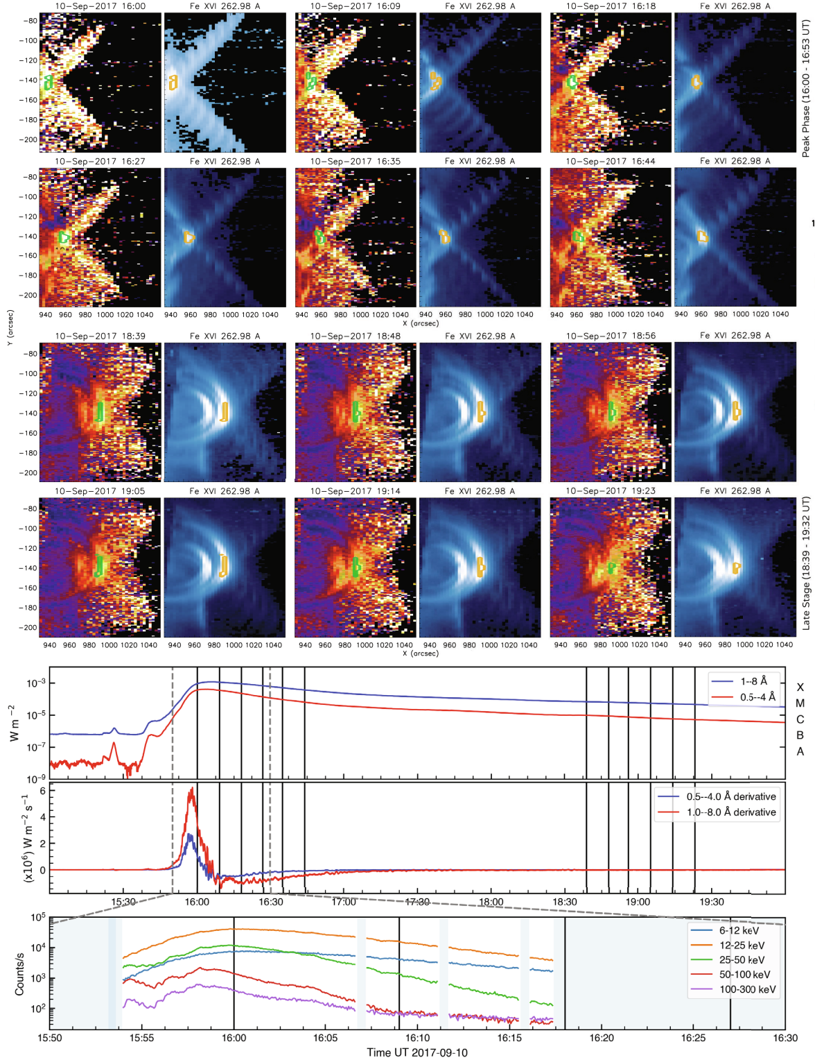
Fig. 1. Evolution of the 2017 September 10 X8.2 flare in the peak phase (16:00–16:53 UT) and late stage (18:39–19:32 UT). The upper panel shows Ca XIV 193.87 Å/Ar XIV 194.40 Å intensity ratio (left) and Fe XVI 262.98 Å (right) intensity maps during the peak phase (16:00–16:53 UT) and late stage (18:39–19:32 UT) of the 2017 September 10 X8.2 flare. The following horizontal panels shows from top to bottom, the GOES X-ray lightcurve of the flare – 1–8 Å flux (blue); and the 0.5–4 Å flux (red); the GOES lightcurve derivative (i.e. following the Neupert effect Neupert 1968) and RHESSI light curves in five energy bands, showing the X-ray evolution during the first 40 minutes. The shaded regions in the RHESSI plot denote times when RHESSI was in nighttime or travelling through the South Atlantic Anomaly (SAA) or when the attenuator was changing. Each vertical black line indicate the starting times of a EIS raster. The upper Ca/Ar intensity ratio maps are saturated at 10 – bright orange or yellow indicates a coronal abundance, and cooler colours like dark blue indicate close to photospheric abundances. It is clear that a coronal abundance is observed at the loop apex across all maps, with photospheric abundances toward the loop footpoints. Green or orange contours indicate the brightest regions in the Fe XVI 262.98 Å intensity maps at each corresponding time. Fe XVI 262.98 Å has a formation temperature at \log T = 6.44 K, similar to the Ca XIV 193.87 Å and Ar XIV 194.40 Å lines used.
