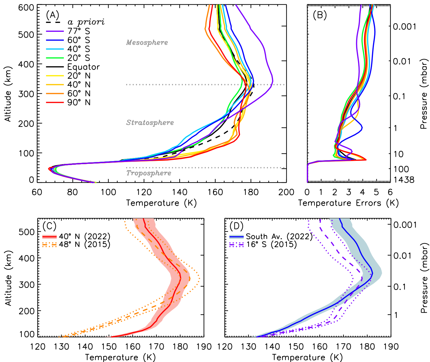
Figure 4. (A) The resulting latitudinally resolved temperature profiles (solid lines) retrieved using the ALMA CO ( J = 6-5 ) spectra. The input disk-averaged profile retrieved from previous ALMA observations (Thelen et al. 2020) is shown (dashed black line). (B) The retrieval errors corresponding to the vertical profiles in panel (A). Errors below \sim 80 km are tapered to 0 K to hold the tropospheric temperature values to those derived from the Cassini Radio Science data (Schinder et al. 2020). (C) Comparison of the retrieved temperature profile from Thelen et al. (2018) over a range of northern latitudes (centered at \sim 48^\circ\text{N} ; dashed orange profile and dotted errors) and the profile presented here at 40^\circ\text{N} (solid red profile and error envelope). (D) Comparison of the retrieved temperature profile from Thelen et al. (2018) representing low southern latitudes ( \sim 16^\circ\text{S} ; dashed purple profile and dotted errors) and an average of the profiles retrieved here from 20^\circ\text{S} to 77^\circ\text{S} (solid blue profile and error envelope). The pressure axis on all panels is approximate, represented by the pressures from equatorial latitudes.
