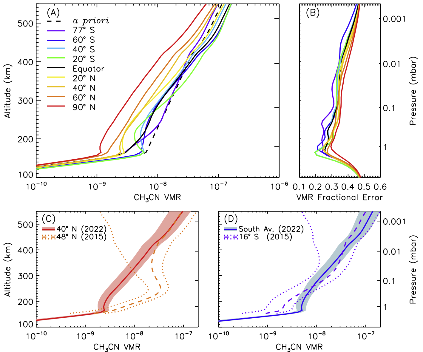
Figure 6. (A) The resulting latitudinally resolved profiles of CH 3 CN abundance (solid lines) retrieved from ALMA CH 3 CN ( J = 38-37 ) spectra. The retrievals are shown in a similar altitude range as the retrieved temperature profiles (Figure 4), though the CH 3 CN spectra are not sensitive to abundance variations below \sim 160 km and above \sim 450 km. The a priori CH 3 CN profile, constructed from the observations by Marten et al. (2002) and photochemical model predictions by Loison et al. (2015), is shown (dashed black line). (B) The fractional VMR error profiles corresponding to the vertical profiles in panel (A). (C) Temporal comparison of the CH 3 CN vertical profile retrieved at 40°N (solid red line and error envelope) to ALMA observations in 2015 (dashed orange profile and dotted errors) from Thelen et al. (2019b). (D) Comparison of an average of southern hemisphere profiles derived here (solid blue line and error envelope) to the vertical profile representing low southern latitudes in 2015 (purple dashed profile and dotted errors) from Thelen et al. (2019b).
