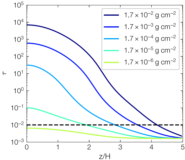
Figure 2. Thermal relaxation time-scale \tau = t_c/P_{\text{orb}} as a function of height, assuming that cooling rate is balanced by photoelectric heating rate of dust grains. Dashed line is the VSI critical thermal relaxation time-scale for h = 0.05 , q = -0.5 , and \gamma = 1.4 at 100 au.
