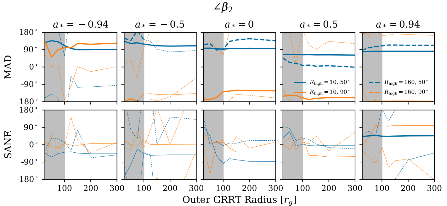
Figure 25. \angle\beta_2 as a function of outer integration radius for a selection of KHARMA models. The GRRT in our work includes material at r \leq 100r_g , encoded by the gray band. Lines transition from thick to thin at the first radius at which |\beta_2| < 0.05 . For models with |\beta_2| > 0.05 , \angle\beta_2 typically converges by r = 100r_g .
