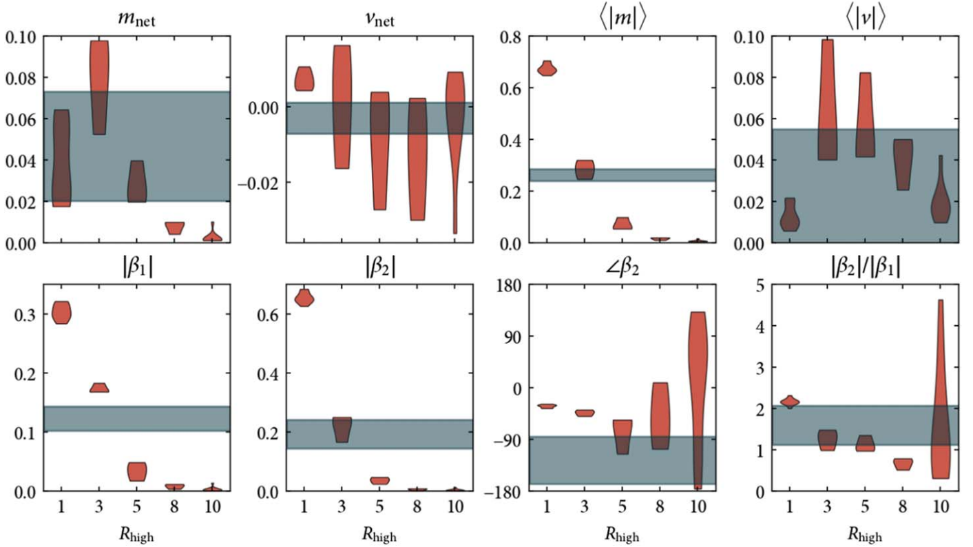
Figure 29. Distributions of observables for a selection of SANE models ray-traced with greater resolution in R_{\text{high}} between 1 and 10. These correspond to KHARMA SANE a_* = -0.5 , i = 150^\circ aligned models. We find rapid evolution in this part of parameter space.
