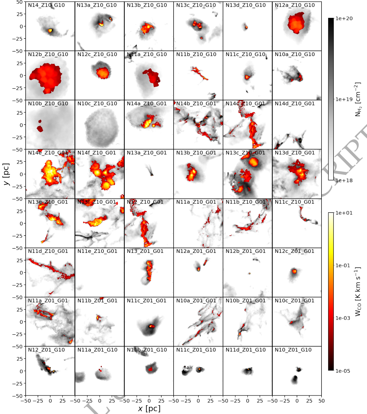
Figure A1. Maps for all of the regions used in the analysis showing W_{\text{CO}} wherever it exceeds 10^{-5} K km \text{s}^{-1} , traced on top of \text{H}_2 surface density. We can see a variety of shapes, sizes and density distributions across the regions, ranging from diffuse “blobs” to dense core-like structures and filaments. Note that the W_{\text{CO}} maps shown here are the direct output from POLARIS, and so the irregular shapes of the Voronoi cells are sometimes apparent.
