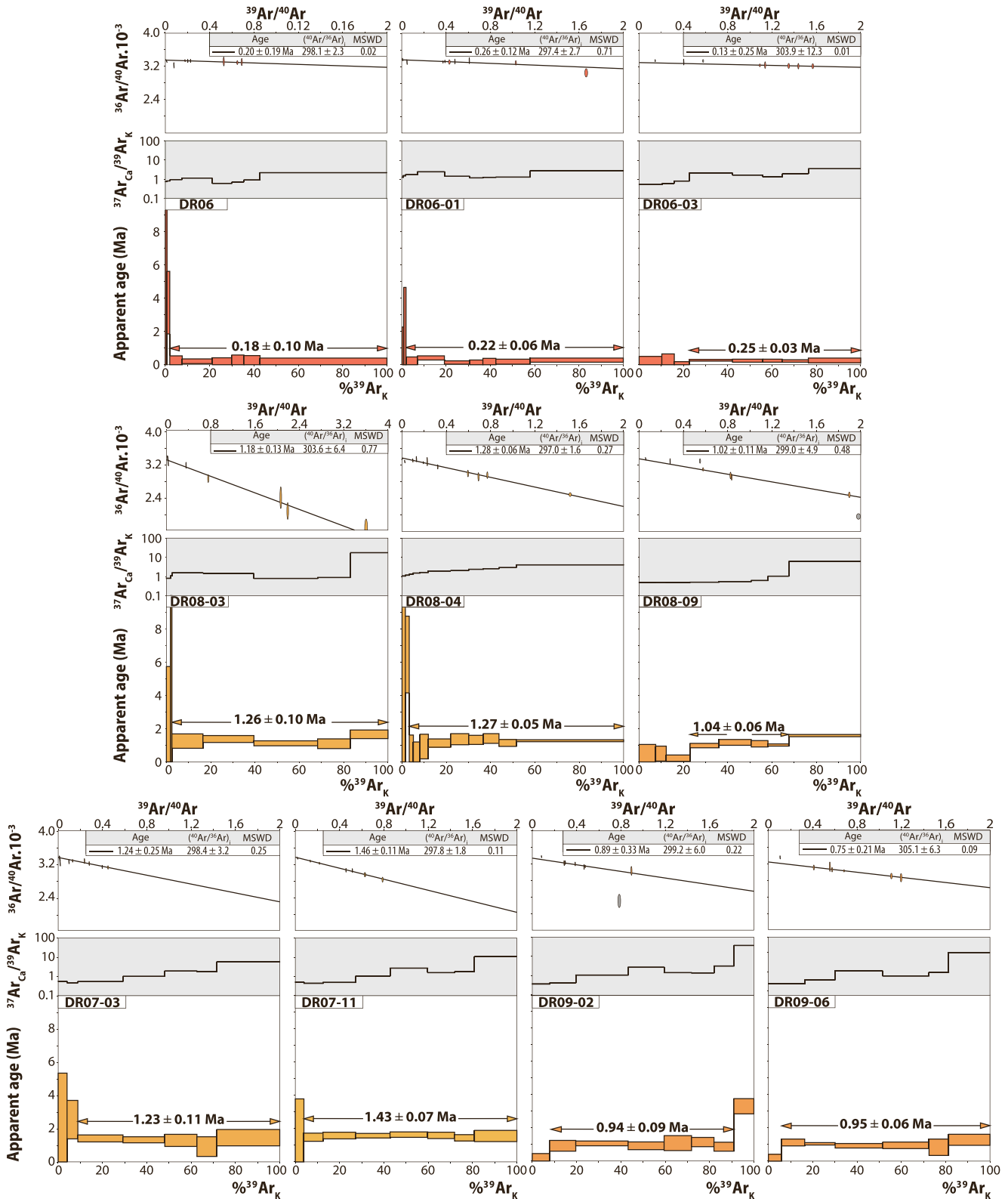
Figure 5. ^{40}\text{Ar}/^{39}\text{Ar} age and ^{37}\text{Ar}_{\text{Ca}}/^{39}\text{Ar}_{\text{K}} spectra of samples from dredges MOZ01-DR06, MOZ01-DR07, MOZ01-DR08 and MOZ01-DR09. Apparent age errors are 1\sigma and do not include errors on the J-parameter. Plateau ages are given with 1\sigma uncertainties including errors in the J-parameter. Inverse isochrons are represented as ^{36}\text{Ar}/^{40}\text{Ar} versus ^{39}\text{Ar}/^{40}\text{Ar} correlation diagrams, excluding gray ellipses from regression (York, 1968; York et al., 2004).
