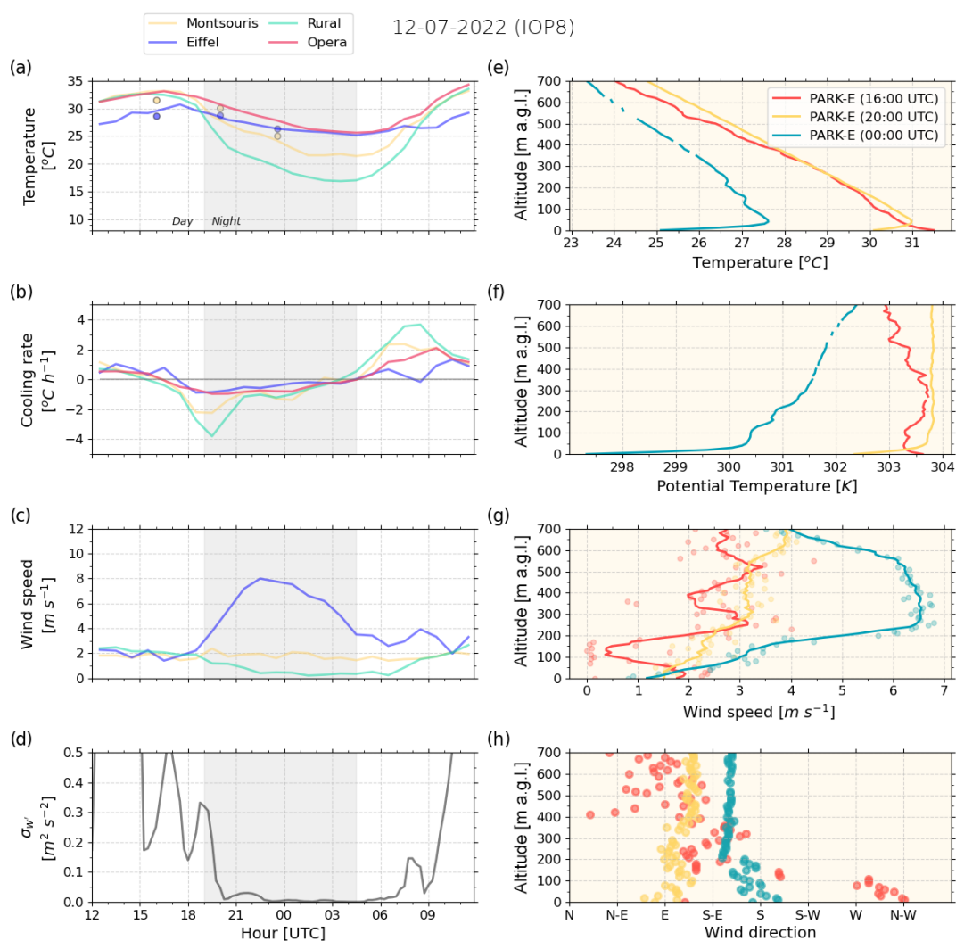
Figure 5. Time series and Windsound profile measurements for 12 July 2022. (a–d) Time series measurements from 12:00 UTC to 12:00 UTC (plus 1 d). (a) Temperature at Montsouris Park, rural settings, Opera (built-up) and the top of the Eiffel Tower. The coloured dots show the temperature measured by Windsonds at 16:00, 20:00 and 00:00 UTC at park level and at the height of the Eiffel Tower (287 m a.g.l.). (b) Cooling rate at Montsouris, rural, Opera and Eiffel Tower sites. (c) Wind speed at Montsouris, rural and Eiffel Tower sites. (d) Vertical velocity variance from DWL at 240 m a.g.l. at the Qualair-SU site. (e–h) Vertical profiles from radiosonde measurements released in PARK-E at 16:00, 20:00 and 00:00 UTC, respectively. (e) Temperature profile. (f) Potential temperature profiles. (g) Wind speed profiles. (h) Wind direction profiles.
