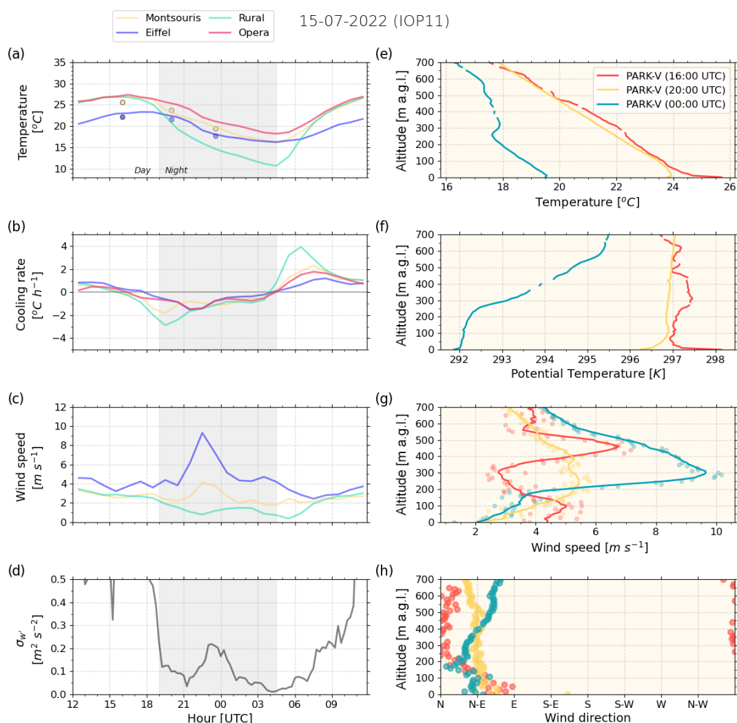
Figure 7. Same as Fig. 5 but for 15 July 2022 (IOP11).
