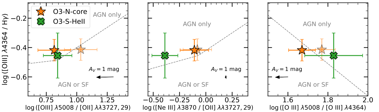
Fig. 6. Diagnostic line-ratio diagrams based on [\text{O III}] \lambda 4364 emission. In all three panels the dashed line is the empirical demarcation between pure AGN and AGN/SF mixtures proposed by Mazzolari et al. (2024). The faded markers with error bars are determined from our pPXF fits to the spectra without reddening correction. The bold markers show the values after reddening correction, with A_V = 1.58 \pm 0.16 mag for O3-N-core and A_V = 0 mag for O3-S-HeII. The black arrows denote the dereddening vector for an attenuation of A_V = 1 mag with the Calzetti et al. (2000) attenuation law.
