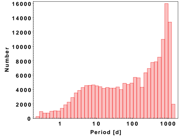
Fig. 25. Histogram of the observed period distribution. We note that the period is on a logarithmic scale.
