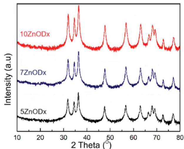
Figure 1: The XRD patterns of dextran coated zinc oxide samples.
