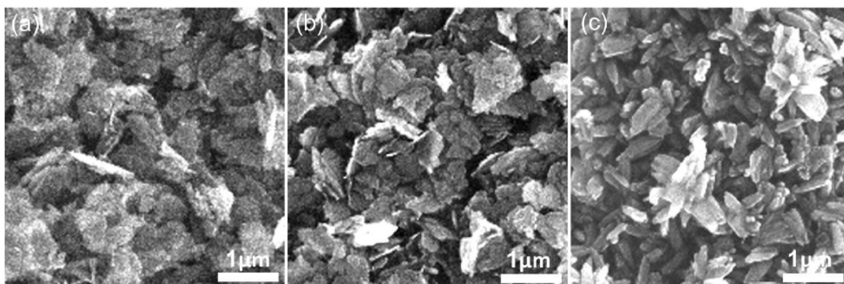
Figure 2: SEM micrographs of 5ZnODx (a), 7ZnODx (b) and 10ZnODx (c).
