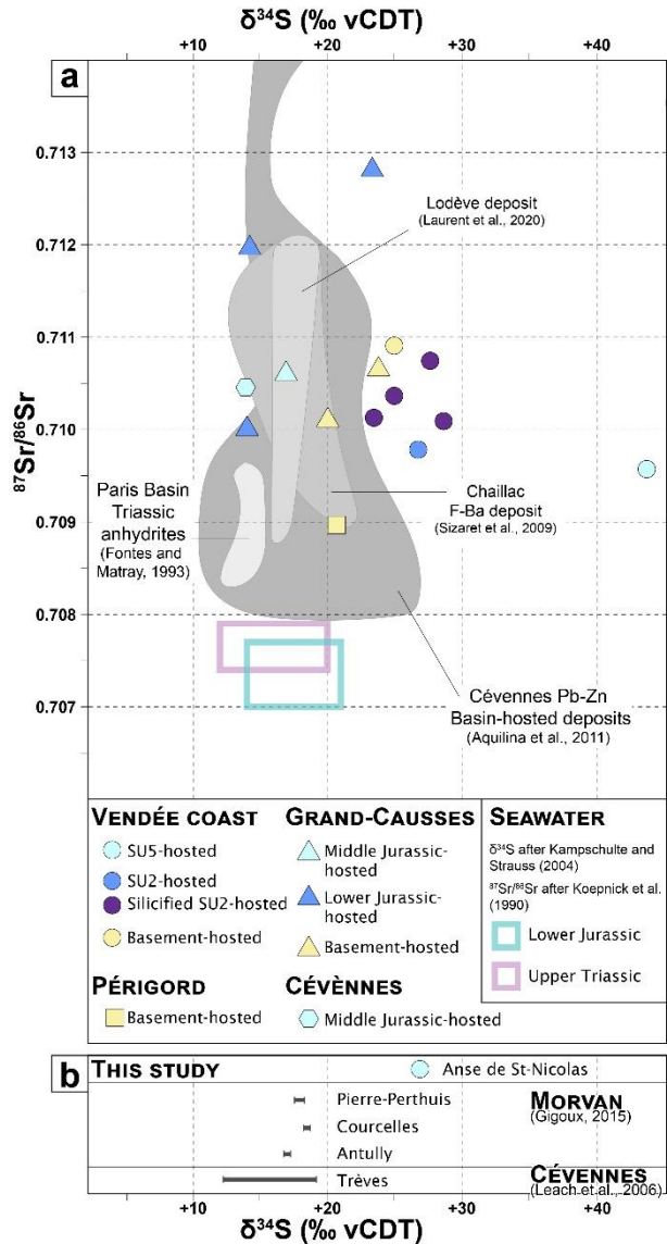
Figure 5. a: ^{87}\text{Sr}/^{86}\text{Sr} vs \delta^{34}\text{S} plot for Brt4-baryte samples from the Vendée coast and baryte samples from other districts (see Table 1). Shaded area and boxes represent literature data. b: \delta^{34}\text{S} plot for baryte samples. Brt4-baryte samples correspond to the SU5 sample from Anse de St-Nicolas (see Table 1).
