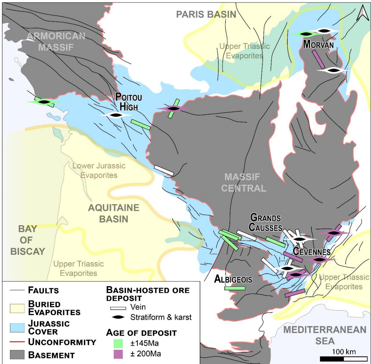
Figure 8. Simplified geological map of France with basin-hosted ore deposits. See Table 2 for details and references about deposits age. The Upper Triassic and Lower Jurassic map of the buried evaporites from Curnelle and Dubois (1986) and Mégnien et al. (1980).
