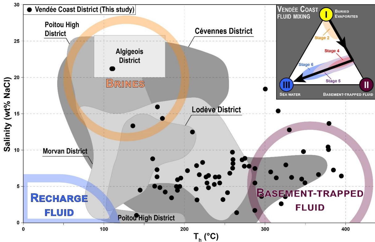
Figure 7. Salinity-Temperature diagram of FIs from ore deposits in French basin (See Table 2 for references).
