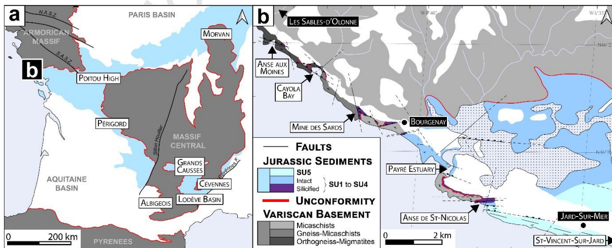
Figure 1. Location of unconformity-related ore deposits between Variscan massifs and Jurassic sediments
