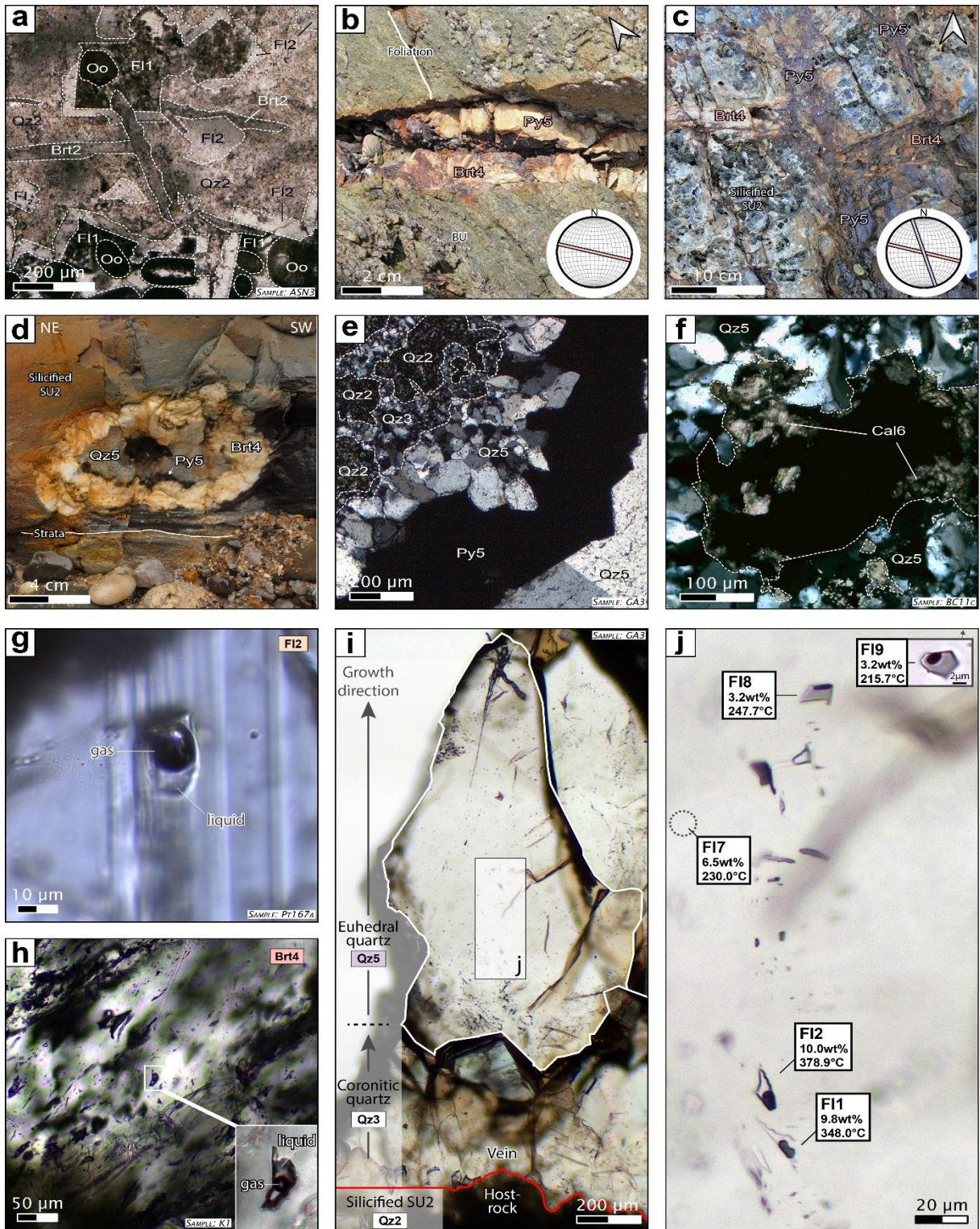
Figure 3. a: Disseminated F11-fluorite in association with epigenized oolites (Oo) with F12 overgrowth, F12-fluorite crystals, Brt2 in needle-shape and cryptocrystalline Qz2 hosted in SU2. b: Basement-hosted WNW-ESE Brt4-baryte vein. c: WNW-ESE Brt4-baryte vein hosted in SU2- and crosscut by NNW-SSE Py5-pyrite vein. d: karst filled by Brt4-baryte, Py5-pyrite and Qz5-quartz hosted in SU2. e:
