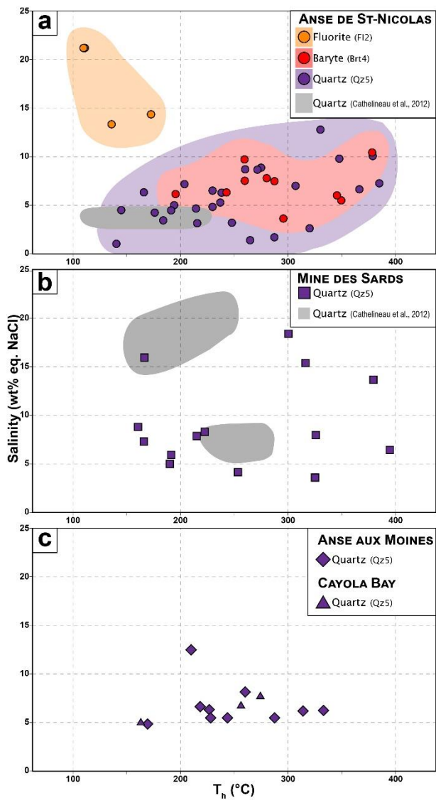
Figure 4. Salinity vs T_h diagram for FIs from (a) Anse de St-Nicolas, (b) Mine des Sardes and (c) Anse aux Moines and Cayola Bay (Table 1).
