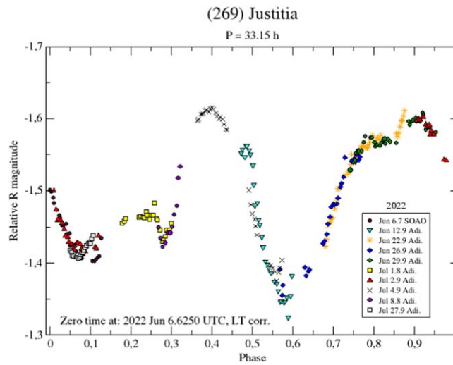
Figure 6. Composite lightcurve of (269) Justitia from the year 2022.
