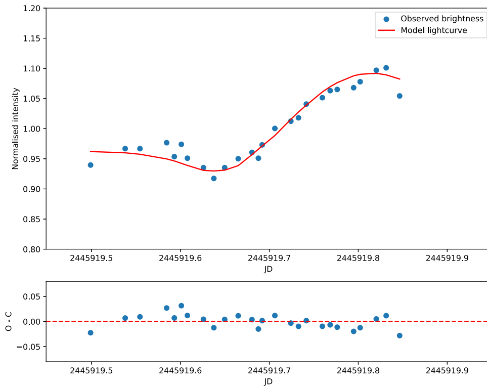
Figure 7. Example fit of Justitia model to visible lightcurves. Due to a slow rotation (33 hr period), each lightcurve covers only a small portion of the full period. (The data used to create this figure are available in the online article .) (The complete figure set (51 images) is available in the online article .)
