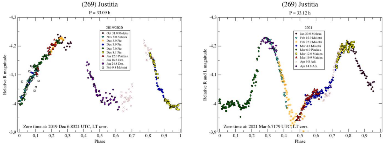
Figure 5. Composite lightcurves of (269) Justitia from the verge of the years 2019 and 2020 (left) and from the year 2021 (right).
