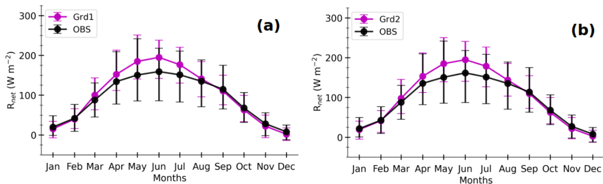
Figure A6. Composite monthly averages of simulated surface net radiative flux ( R_{net} , magenta lines) at Grd1 (a) and Grd2 (b) and those of their respective observations at Météopole (black lines). They are computed as in Fig. 13.
