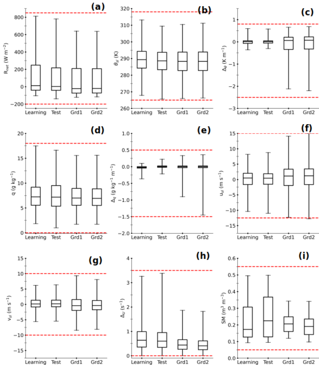
Figure A1. Box plots summarizing the interval ranges of the nine physical variables used as input to our MLP-based statistical model (Table 2). The corresponding datasets are indicated on the x axis. The whiskers represent the minimum and maximum values of each dataset. The horizontal dashed red lines indicate the extreme values used for scaling.
