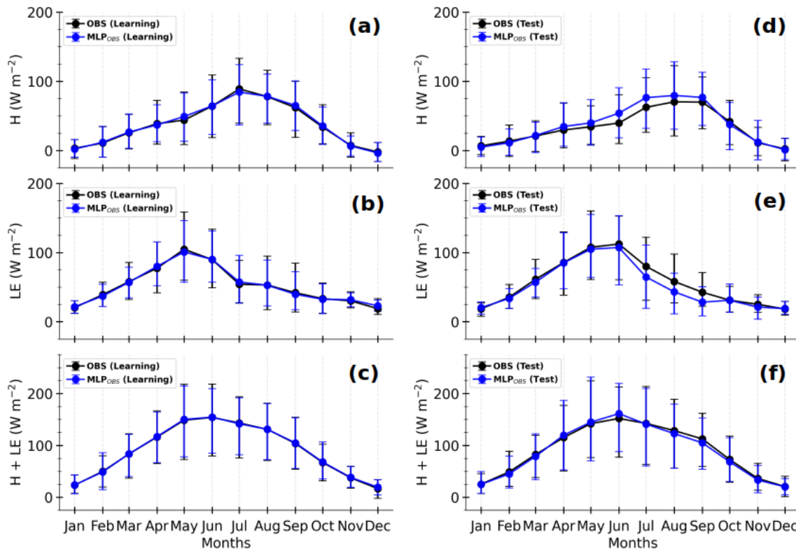
Figure 8. Composite monthly averages of observed (OBS in black) and MLP-based ( \text{MLP}_{\text{OBS}} in blue) sensible heat flux ( H , a, d), latent heat flux ( LE , b, e), and total turbulent heat flux ( H + LE , c, f) for the learning (a–c) and test sets (d–f) respectively. The solid lines represent the means, and the error bars correspond to the 10th and 90th percentiles, calculated by gathering the daily averages of half-hourly samples in Fig. 6.
