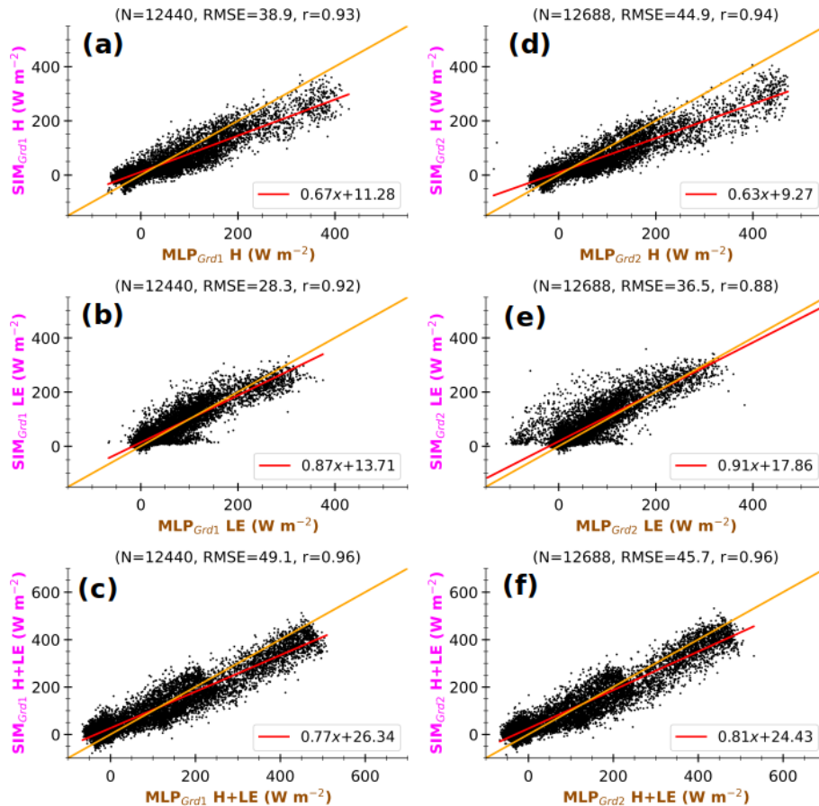
Figure A5. The 3 h simulated sensible heat flux ( H , a, d), latent heat flux ( LE , b, e), and total turbulent heat flux ( H+LE , c, f) at Grd1 (a–c) and Grd2 (d–f) against corresponding MLP-based estimates in the simulated environment. All selected timestamps from 1 January 2012 to 31 December 2016 are considered here. The values at the top of each panel correspond to the number of samples ( N ), root mean square error (RMSE), and Pearson’s correlation coefficient ( r ). The lines in red and orange represent the linear and ideal fits respectively. The axis labels are colored according to the schematic illustration in Fig. 1.
