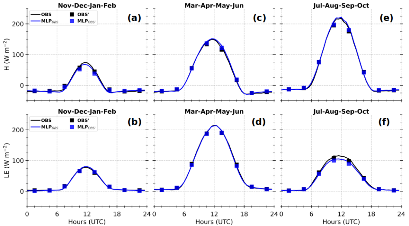
Figure 9. Composite diurnal cycles of half-hour and 3 h observed heat fluxes (OBS and OBS', in black) and their competing MLP-based estimates (MLP OBS and MLP OBS' respectively, in blue), for H (a, c, e) and LE (b, d, f), by splitting the annual cycle into three typical sub-periods (see the text for more details). They are calculated based on diurnal cycles where at least six out of eight expected OBS' samples are available (approximately 85% of all selected diurnal cycles).
