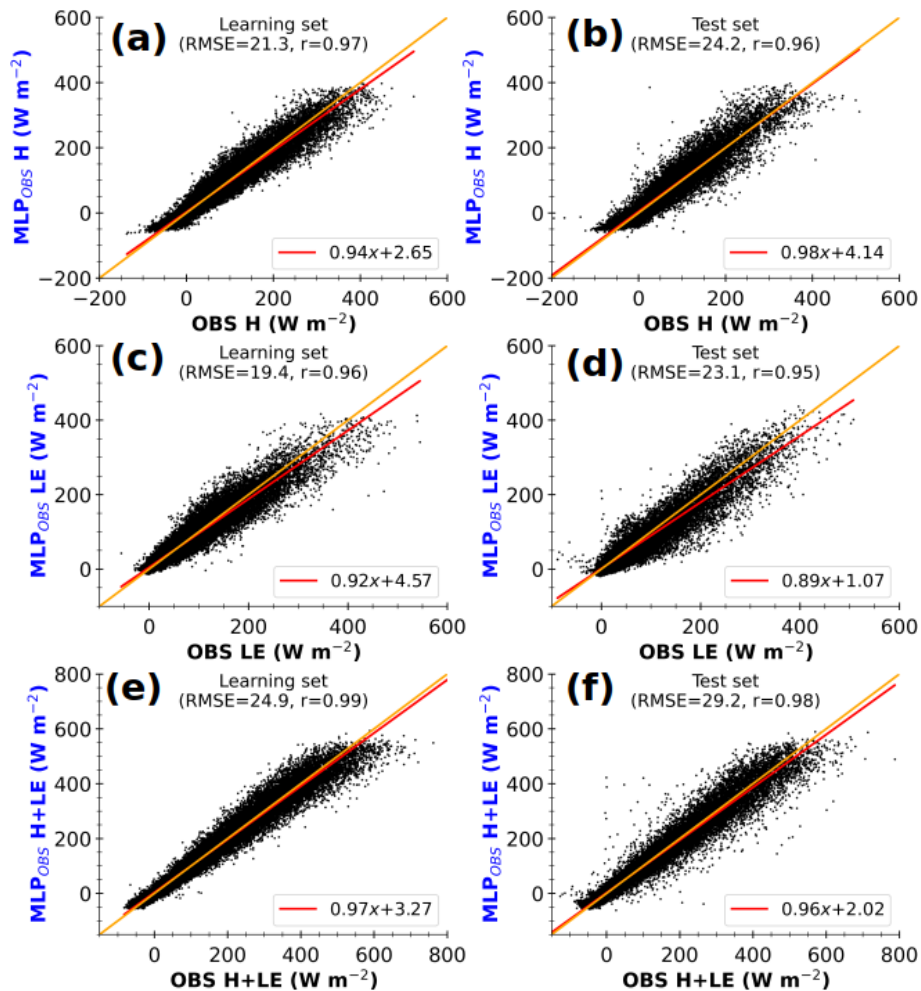
Figure 6. Half-hourly MLP-based estimates of observed sensible heat flux ( MLP_{OBS} H , a, b), latent heat flux ( MLP_{OBS} LE , c, d), and total turbulent heat flux ( MLP_{OBS} H + LE , e, f) with observed input data against observed fluxes (OBS), for learning (a, c, e) and test (b, d, f) sets. The values at the top of each panel correspond to root mean square error (RMSE) and Pearson's correlation coefficient. The lines in red and orange represent the linear regression and identical fits respectively. The axis labels are colored according to the schematic illustration in Fig. 1 (right side).
