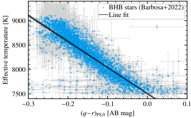
Fig. B.1. Correlation of (g-r)_{\text{PS},0} and effective temperature among BHB stars in the Barbosa et al. (2022) sample (probability of being BHB star of 100 per cent)
