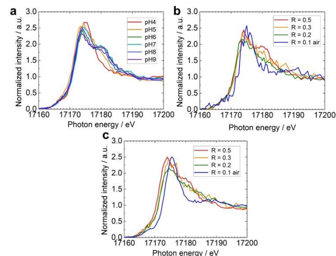
Figure 2. U L 3 -edge HERFD-XANES spectra of U reacted with (a) stoichiometric magnetite (R=0.5) nanoparticles at different pH, (b) magnetites with different stoichiometries at pH 6 and (c) pH 8
