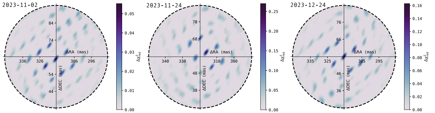
Figure 1. Detections of AF Lep b within the VLTI/GRAVITY fiber field of view. Each panel visualizes the z_{\text{red}} = \Delta\chi_{\text{red}}^2 calculated for various positions ( \Delta R.A. and \Delta Decl. in milliarcseconds, i.e., the displacement with respect to the measured position of the host star AF Lep A), fitting the interferometric observables with a polynomial model of the transmission and stellar halo contribution and a coherent point source with the spectral signature of a T dwarf. Each epoch is presented chronologically, left to right: 2023 November 2, 2023 November 24, and 2023 December 24. The dashed black circle indicates the effective fiber field of view, \sim 60 mas. The origin is the placement of the science fiber on-sky for a given observation, a prediction based on the previous available orbit fit. The strongest peak in the \chi^2 map reveals the position of the companion, with lower likelihood peaks surrounding this central peak. The shape and distribution of the likelihood depend on the u - v plane coverage of the observations.
