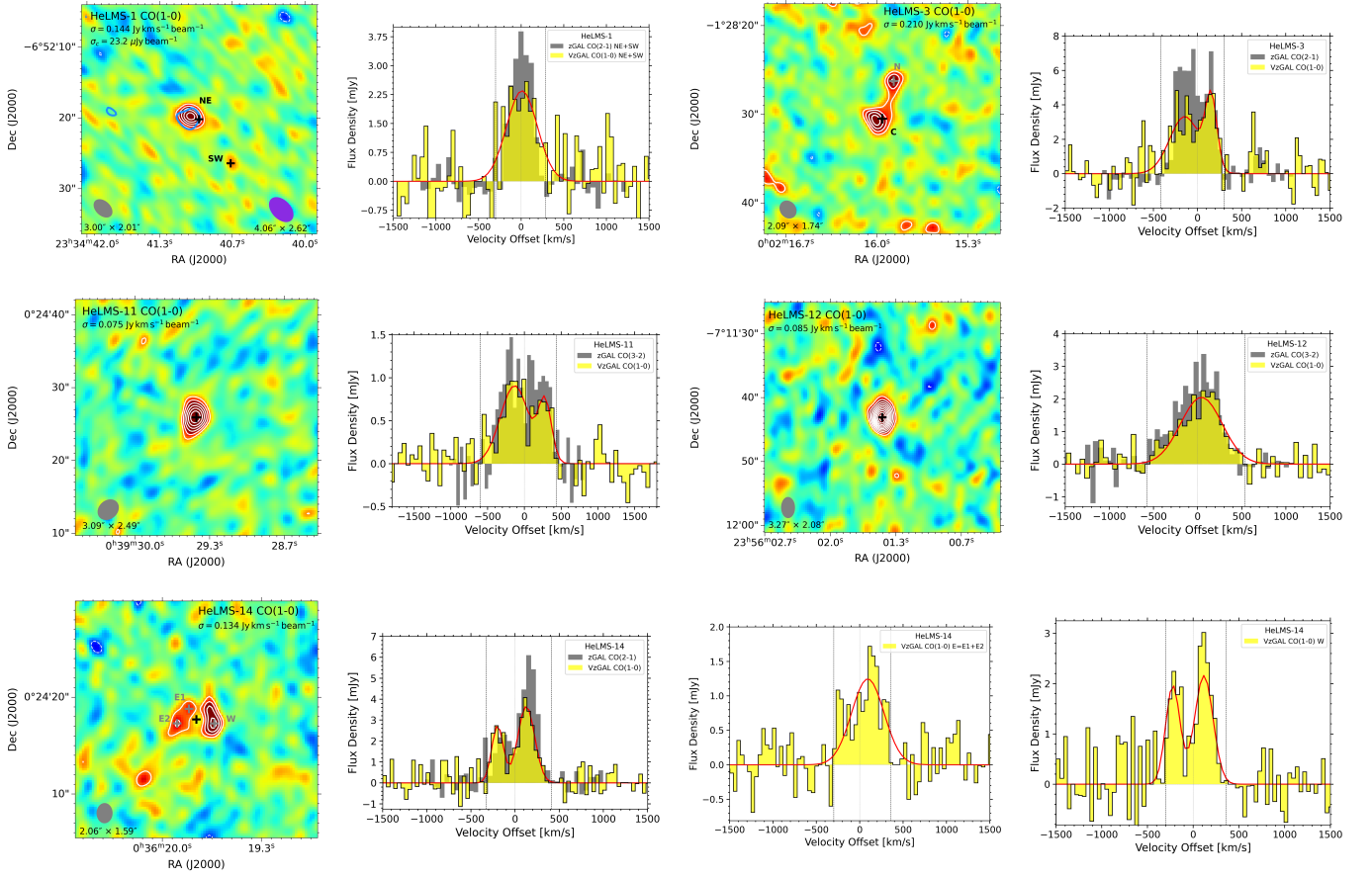
Figure 10. Moment-0 maps and spectra of low- J CO emission, namely CO(1–0) and CO(2–1), of the V_z -GALaxies (HeLMS-1 to HeLMS-48 but HeLMS-47 here). We provide the rms noise ( \sigma ) of each moment-0 map along with the synthesized beam size (gray ellipses) in the image itself. For targets with lensed images or multiplicity, we distinctly add cross-markers identifying different spatial components on these moment-0 maps. Otherwise, the cross markers represent the central position of the DSFG as found in the z -GAL survey (P. Cox et al. 2023). The CO emission is shown using solid/dashed white (positive/negative) contours, starting at \pm 2\sigma . These contours vary in the steps of 1\sigma . For objects with detected continuum emission above 2\sigma_c , we show continuum flux density levels as blue contours. In the cases where we detect a serendipitous radio source along the line of sight or in the field, we show its continuum with magenta contours instead. Please refer to Appendix A (Section A.2) for more details. The synthesized beam (purple ellipses) and noise level ( \sigma_c ) of continuum maps are depicted in the images. The extracted spectra of our CO(1–0) observations (see Section 3.2), depicted in yellow, are compared to higher- J CO lines shown in gray (P. Cox et al. 2023). For 10 V_z -GAL DSFGs with additional CO(2–1) detection, we also present the CO(2–1) spectra alongside the CO(1–0) and higher- J CO lines. Each line spectra from V_z -GAL detections is fitted with Gaussian profile(s) as red curves, with their fitting parameters shown in Appendix A (Tables 3 and 4). The spectra in gray are scaled to 1.5\times the peak of the yellow spectrum. Black vertical dashed lines over the extracted spectra indicate the velocity range over which the moment-0 map of the CO line was integrated. Spectra of individual spatial components of lensed/multiple DSFGs are also depicted, wherever applicable.
