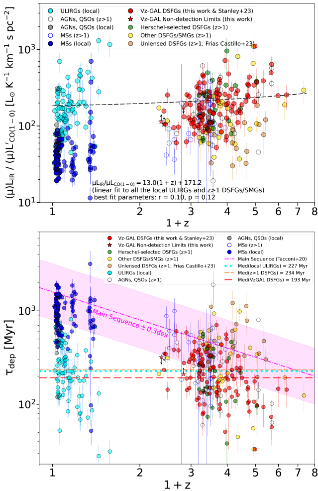
Figure 3. Upper panel: redshift evolution of the total infrared (8–1000 \mu\text{m} ) to CO(1–0) luminosity ratio L_{\text{IR}}/L_{\text{CO}}(1-0) as a proxy for SFE. The linear fit shown with a dashed black line considers all of the high- z DSFGs and local ULIRGs, which shows no confirmation of a linear trend. We choose to plot the redshift in log-scale here to highlight the variation across MS galaxies and ULIRGs at z \sim 0 . Lower panel: variation of the gas depletion time ( \tau_{\text{dep}} ) as a function of redshift when assuming M_{\text{H}_2} = 4L_{\text{CO}}(1-0) (see Section 3.2.1) and \text{SFR} = 1.09 \times 10^{-10} L_{\text{IR}} (see Section 4.2). The dashed red line is the median \tau_{\text{dep}} for the V _z -GAL sources, which is compared to that of local ULIRGs (cyan dotted line) and all DSFGs including the V _z -GAL sample (dashed orange line). The SFR- M_* main sequence (MS) shown as magenta dashed line is based on Figure 7 from L. J. Tacconi et al. (2020), which varies as \tau_{\text{dep}} = 1.6 \times (1+z)^{-1} . Both panels include the literature data points mentioned in the caption of Figure 2. Please note that a gap in CO(1–0) observations (rest-frame 115 GHz) around z = 1 is due to the current observational limitation at corresponding redshifted frequencies.
