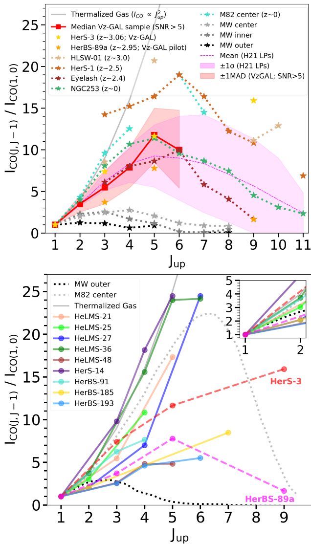
Figure 5. Upper panel: median CO SLED of the V z -GAL sample (solid red curve) compared to sources from the literature including: five high-z DSFGs, HerS-3 at z = 3.061 (this work and P. Cox et al. 2025), HerBS-89a at z = 2.95 (S. Berta et al. 2021), HLSW-01 at z = 2.96 (D. A. Riechers et al. 2011c; K. S. Scott et al. 2011), HerS-1 at z = 2.55 (K. C. Harrington et al. 2019; B. Liu et al. 2022), and the Cosmic Eyelash at z = 2.32 (A. L. R. Danielson et al. 2011; A. M. Swinbank et al. 2011); local starbursts NGC 253 (F. P. Israel et al. 1995; M. J. F. Rosenberg et al. 2014; J. P. Pérez-Beaupuits et al. 2018) and M82 center (A. Weiß et al. 2005b); and the Milky Way, where we adopted the line fluxes of three different regions from D. J. Fixsen et al. (1999), namely the central star-forming zone (MW center), the inner disk (MW inner), and the outer disk (MW outer). The magenta-shaded region is based on the model-derived median line ratios of Planck-identified lensed galaxies (H21 LPs; K. C. Harrington et al. 2021), which is in good agreement with our V z -GAL median values (region shaded in red). Lower panel: CO SLEDs of 11 individual high-z DSFGs from our V z -GAL sample in comparison with the Milky Way and local starburst M82. This plot highlights the variety of excitation conditions across the V z -GAL large sample. SLED modeling for two of these galaxies, namely HerS-3 and HerBS-89a, has already been presented by P. Cox et al. (2025) and S. Berta et al. (2021), respectively. The gray solid curve in both panels shows optically thick and thermalized gas condition of the CO SLED. All of the line fluxes ( I_{\text{CO}} ) used here are in the units of \text{Jy km s}^{-1} .
